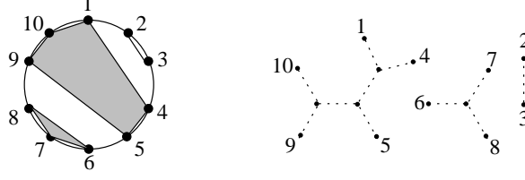
FIGURE 3.1. The Riordan tree associated to the Riordan partition \{\{1, 4, 5, 9, 10\}, \{2, 3\}, \{6, 7, 8\}\} .
