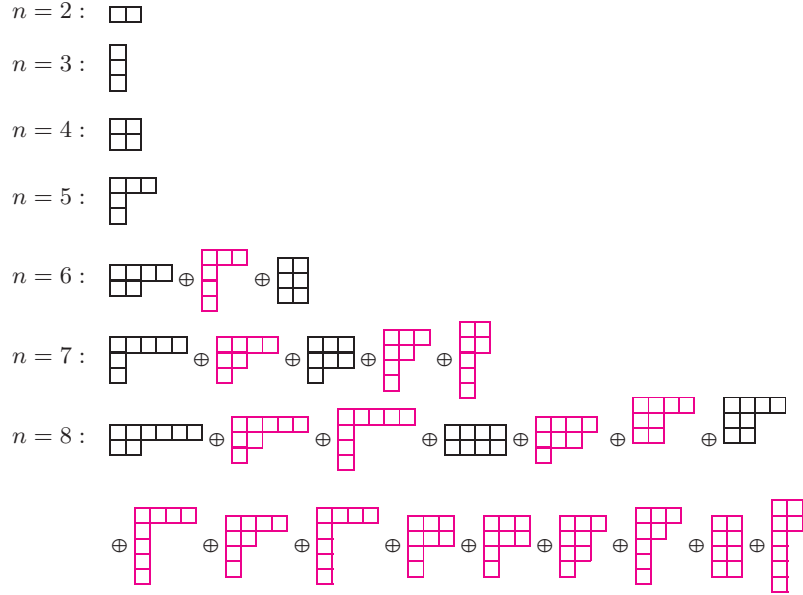
FIGURE 3.3. Irreducible decompositions of \mathcal{C}_n , 2 \leq n \leq 8 , as \mathfrak{S}_n -modules. The red components are in the kernel of W_n^h .
