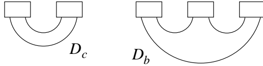
FIGURE 4.2. FK diagrams representing the dual canonical bases for \text{Inv}_{U_q}(V_2^{\otimes 2}) and \text{Inv}_{U_q}(V_2^{\otimes 3}) .
