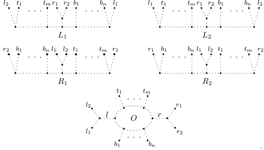
FIGURE 3.4. The diagrams L_1, L_2, R_1, R_2 and O ; here m, n \geq 0 are such that k = (m + n + 2)/2 .
