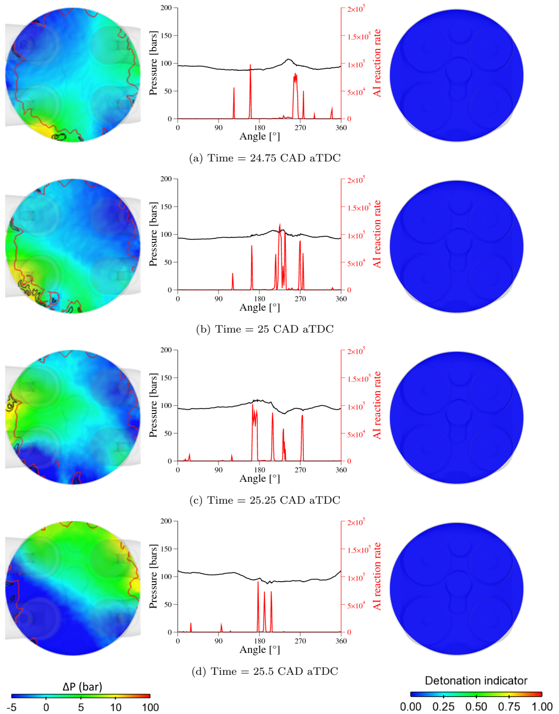
Figure 14: \Delta P evolution (left, red line: isoline of c_{\Sigma} ; black line: isoline of c_{ai} ), pressure and AI reaction rate on the 1D profile (middle) and detonation indicator \mathbb{R} (right) for cycle 8 at ST = 0 CAD.
