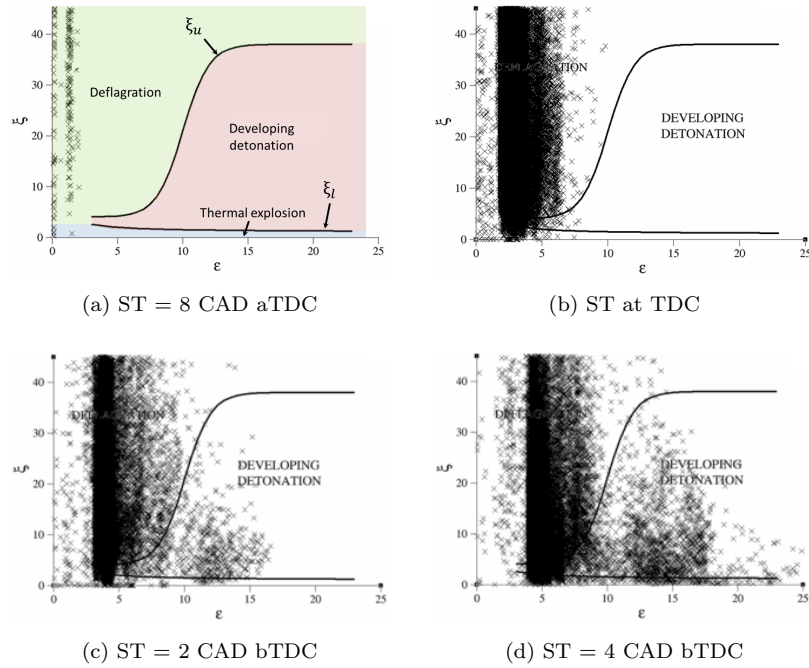
Figure 5: Scatterplot of grid nodes close to autoignite in the detonation diagram.
