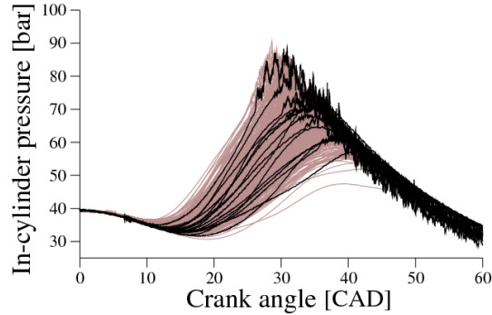
Figure 2: Local in-cylinder pressure with a spark ignition at 6 CAD aTDC [13].
