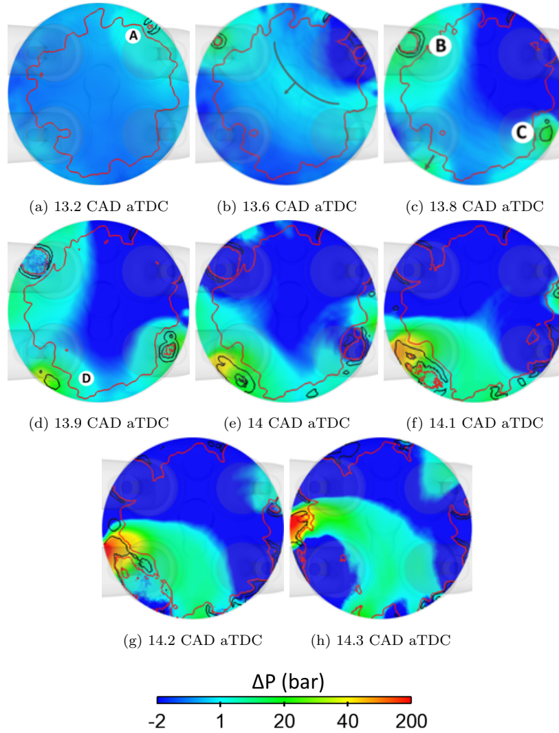
Figure 16: \Delta P visualizations for cycle 7 at ST = 4 CAD bTDC (Red line: isoline of c_\Sigma ; Black line: isoline of c_{ai} ).
