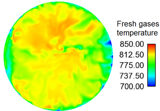
(a) Fresh gases temperature field
