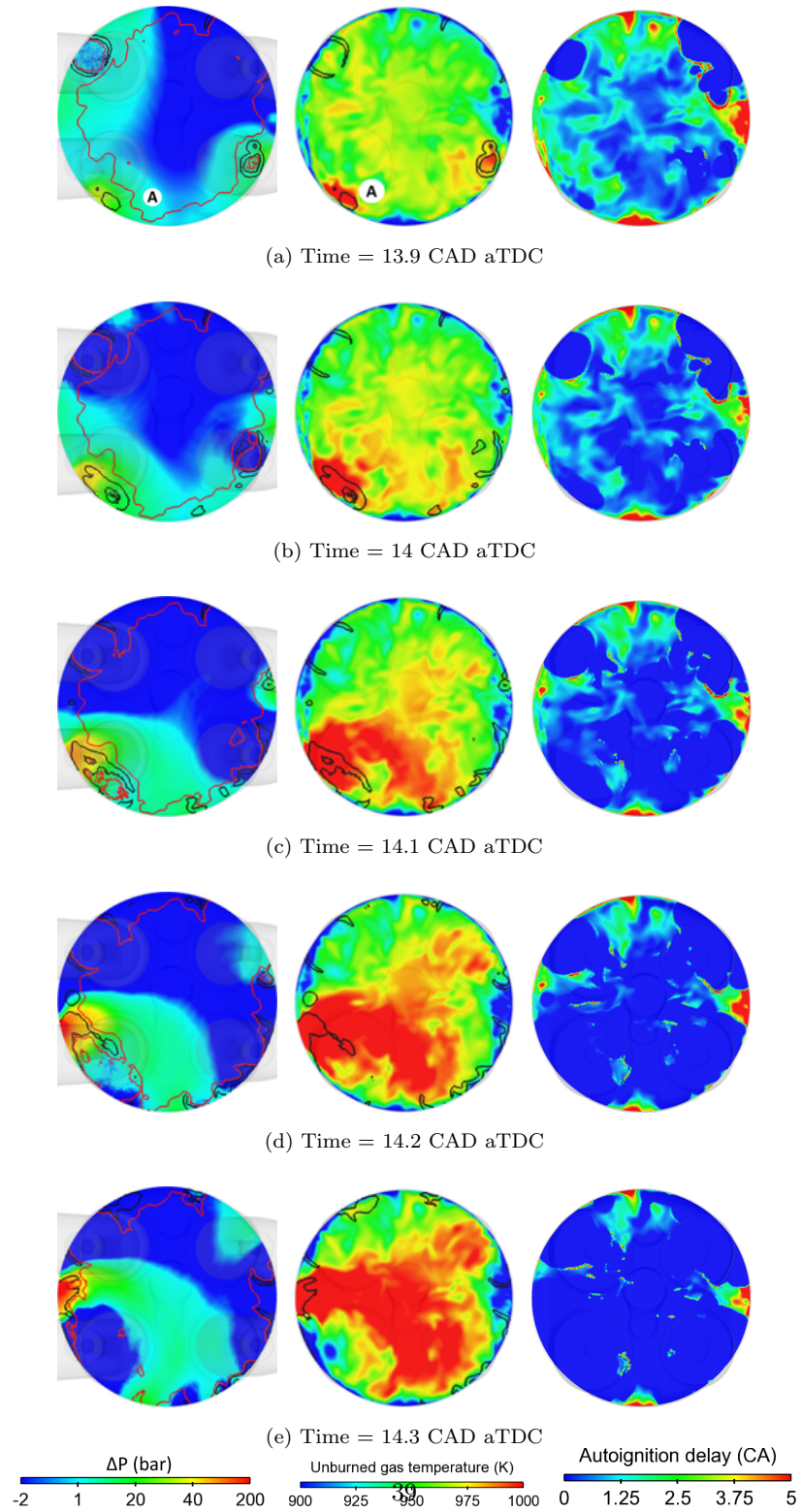
Figure 17: \Delta P evolution (left), fresh gases temperature (middle) and AI delay (right) at several instants where a DDT is supposed for cycle 7 at ST = 4 CAD bTDC (Red line: isoline of c_{\Sigma} ; Black line: isoline of c_{ai} ).
