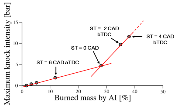
Figure 4: Evolution of the maximum knock intensity over the percentage of mass burned by autoignition for the LES spark timing sweep.
