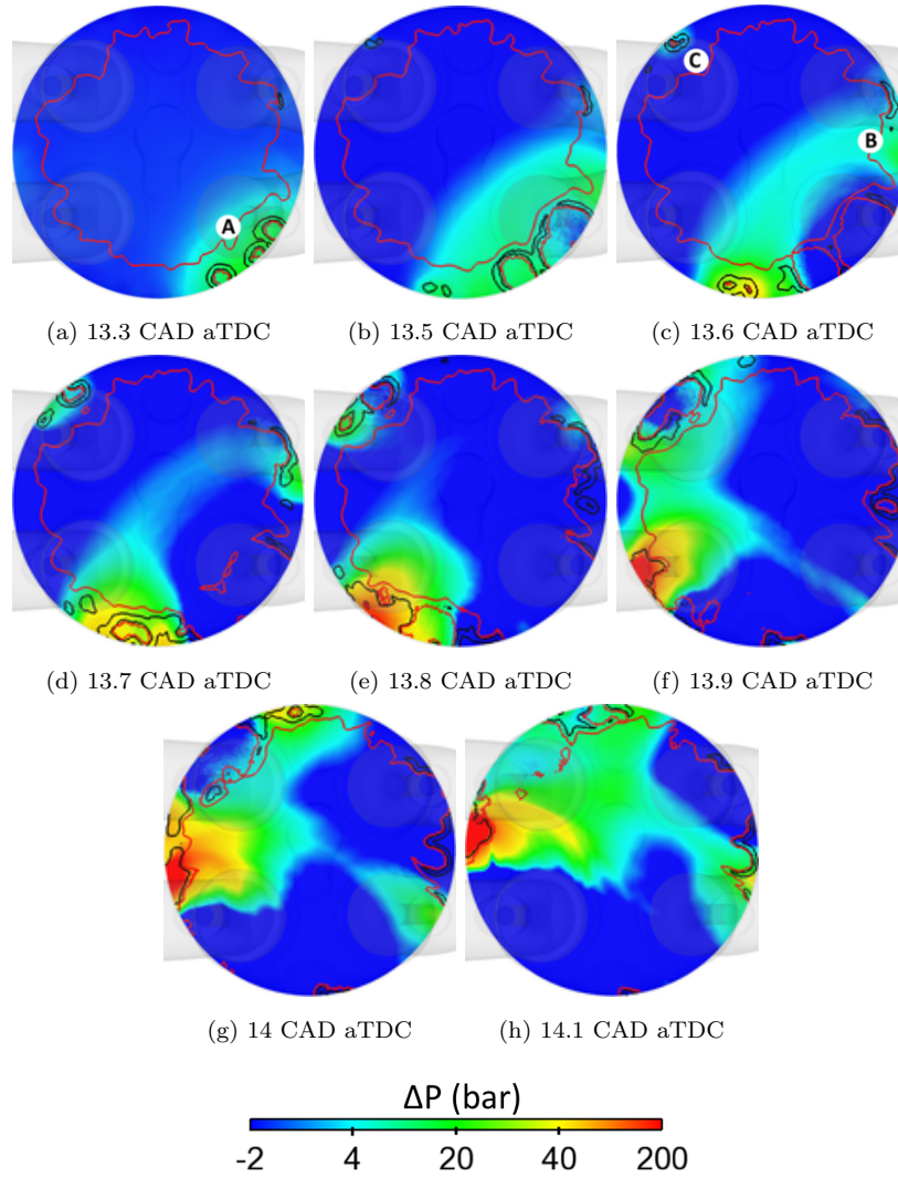
Figure 19: \Delta P evolution for cycle 8 at ST = 4 CAD bTDC (Red line: isoline of c_\Sigma ; Black line: isoline of c_{ai} ).
