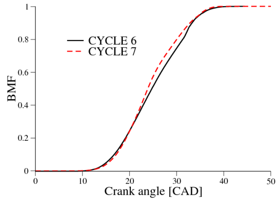
(a) Burned mass fraction
