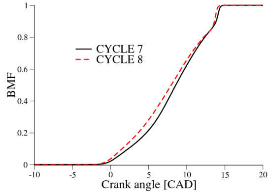
(a) Burned mass fraction over CAD
