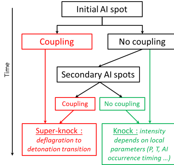
Figure 21: Schematization of AI scenarii visualized in LES calculations.
