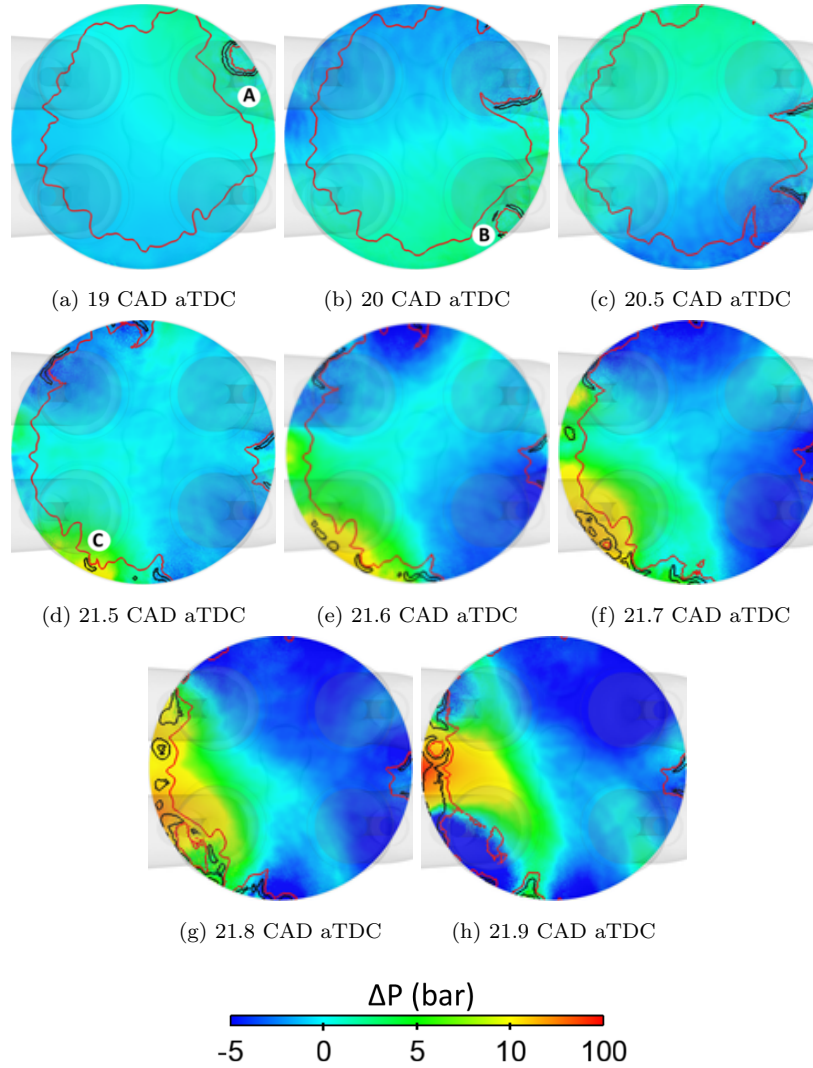
Figure 10: \Delta P evolution for cycle 6 at ST = 0 CAD (Red line: isoline of c_{\Sigma} ; Black line: isoline of c_{ai} ).
