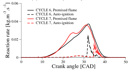
(c) Fuel reaction rates
