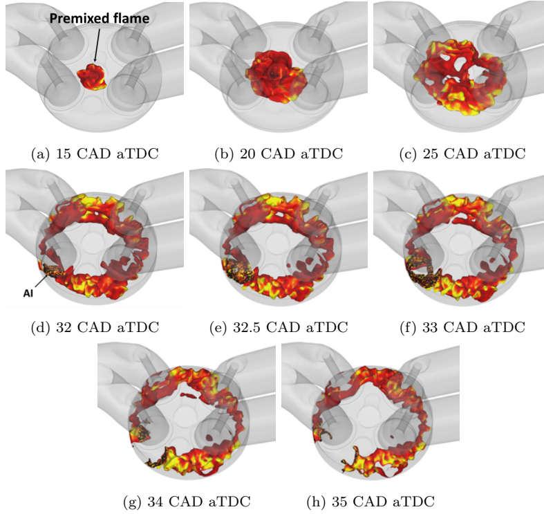
Figure 7: Evolution of 3D isosurfaces of \tilde{c}_\Sigma (yellow/red), and c_{ai} (black) for cycle 6 at ST = 8 CAD aTDC.
