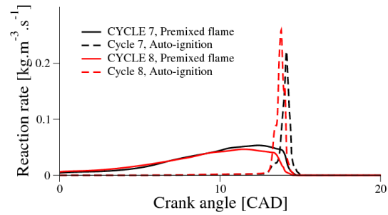
(c) Fuel reaction rates over CAD
