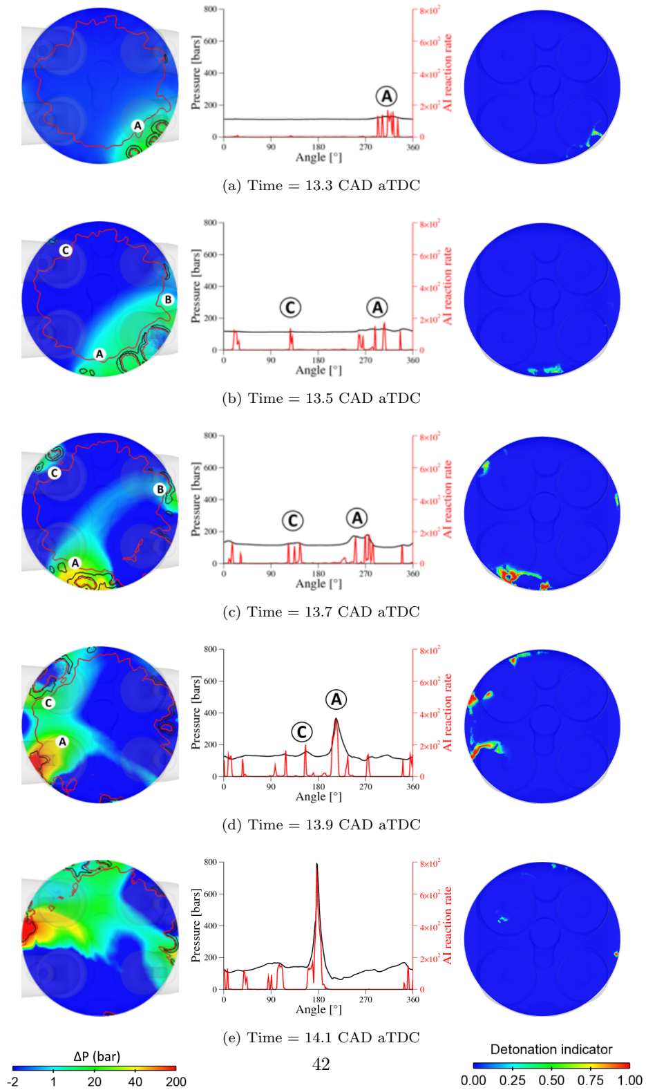
Figure 20: \Delta P evolution (left, red line: isoline of c_{\Sigma} ; black line: isoline of c_{ai} ), pressure and AI reaction rate on the 1D profile (middle) and detonation indicator (right) at several instants where a DDT is established for cycle 8 at ST = 4 CAD bTDC.
