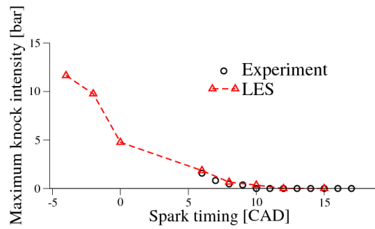
(b) Full ST sweep
