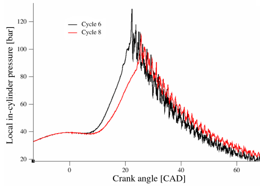
(b) Local in-cylinder pressure over CAD
