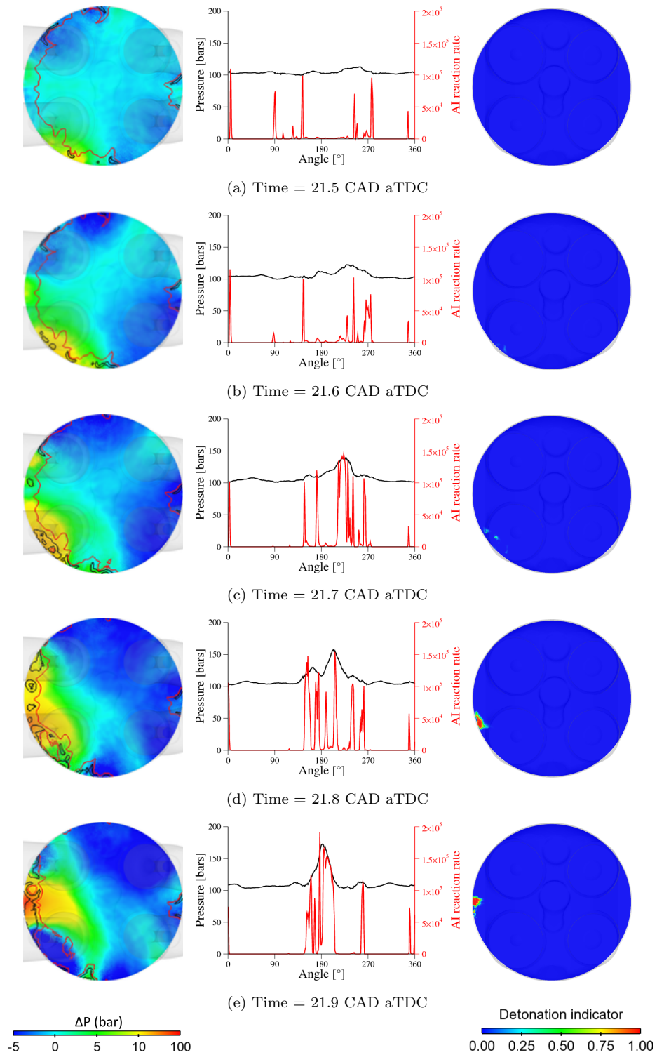
Figure 12: \Delta P evolution (left, red line: isoline of c_{\Sigma} ; black line: isoline of c_{ai} ), pressure and AI reaction rate on the 1D profile (middle) and detonation indicator (right) at several instants where a DDT is supposed for cycle 6 at ST = 0 CAD.
