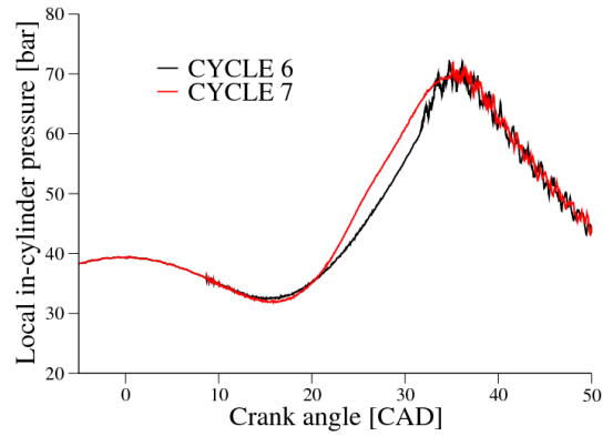
(b) Local in-cylinder pressure
