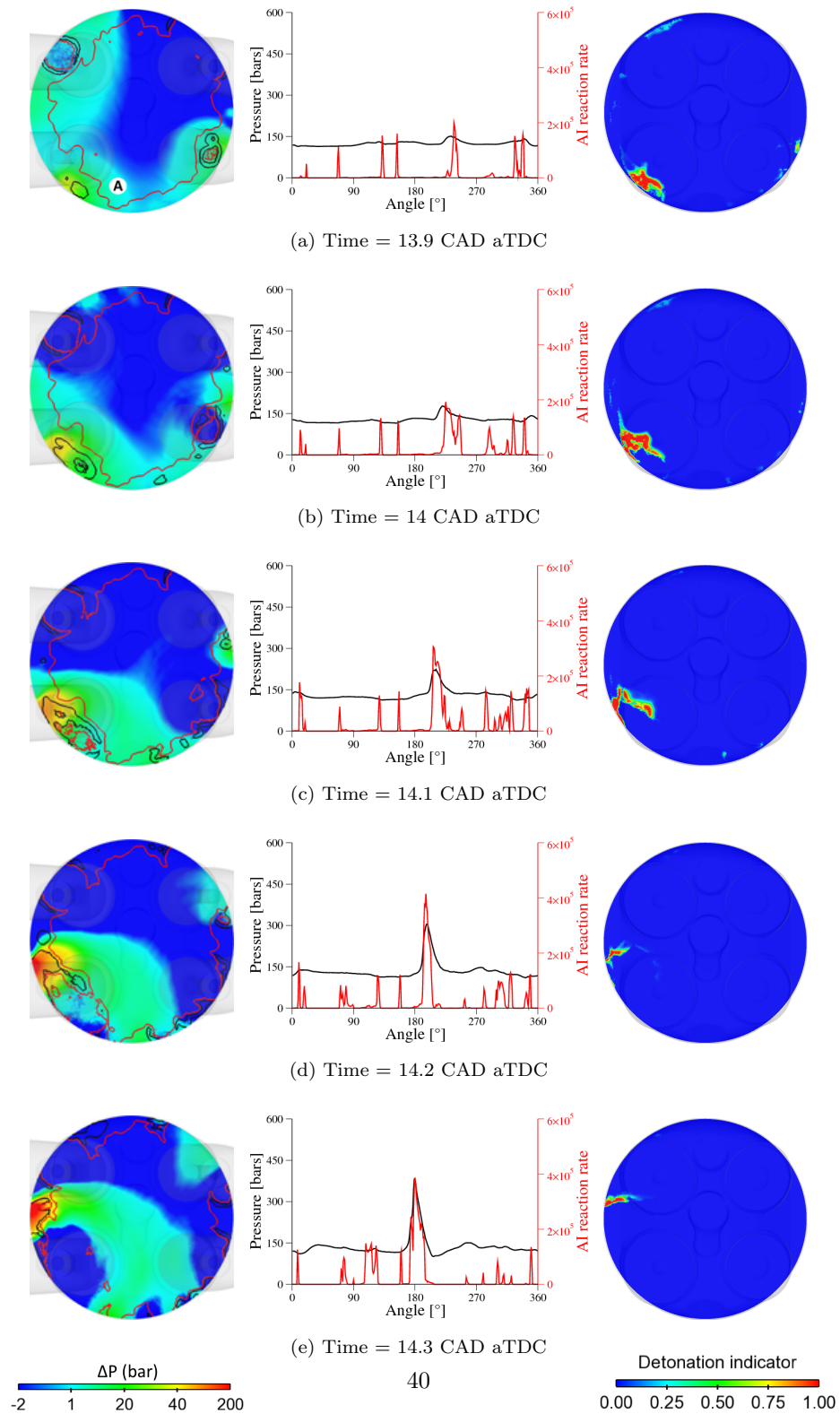
Figure 18: \Delta P evolution (left, red line: isoline of c_{\Sigma} ; black line: isoline of c_{ai} ), pressure and AI reaction rate on the 1D profile (middle) and detonation indicator (right) at several instants where a DDT is supposed for cycle 7 at ST = 4 CAD bTDC.
