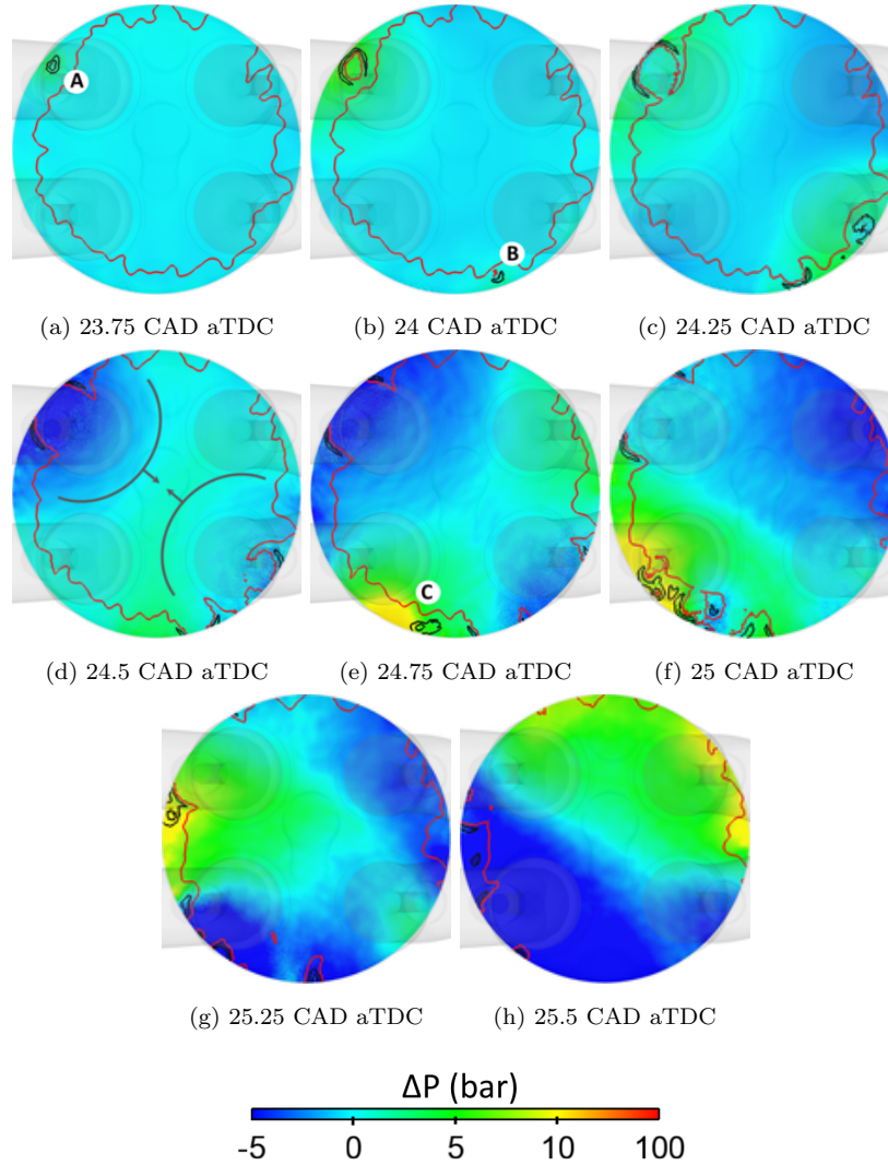
Figure 13: \Delta P visualizations for cycle 8 at ST = 0 CAD (Red line: isoline of c_\Sigma ; Black line: isoline of c_{ai} ).
