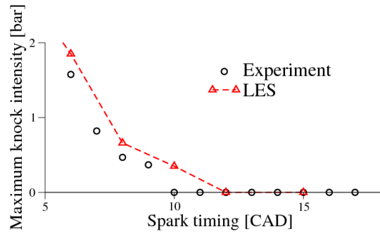
(a) Focus on common ST between LES and experiment
