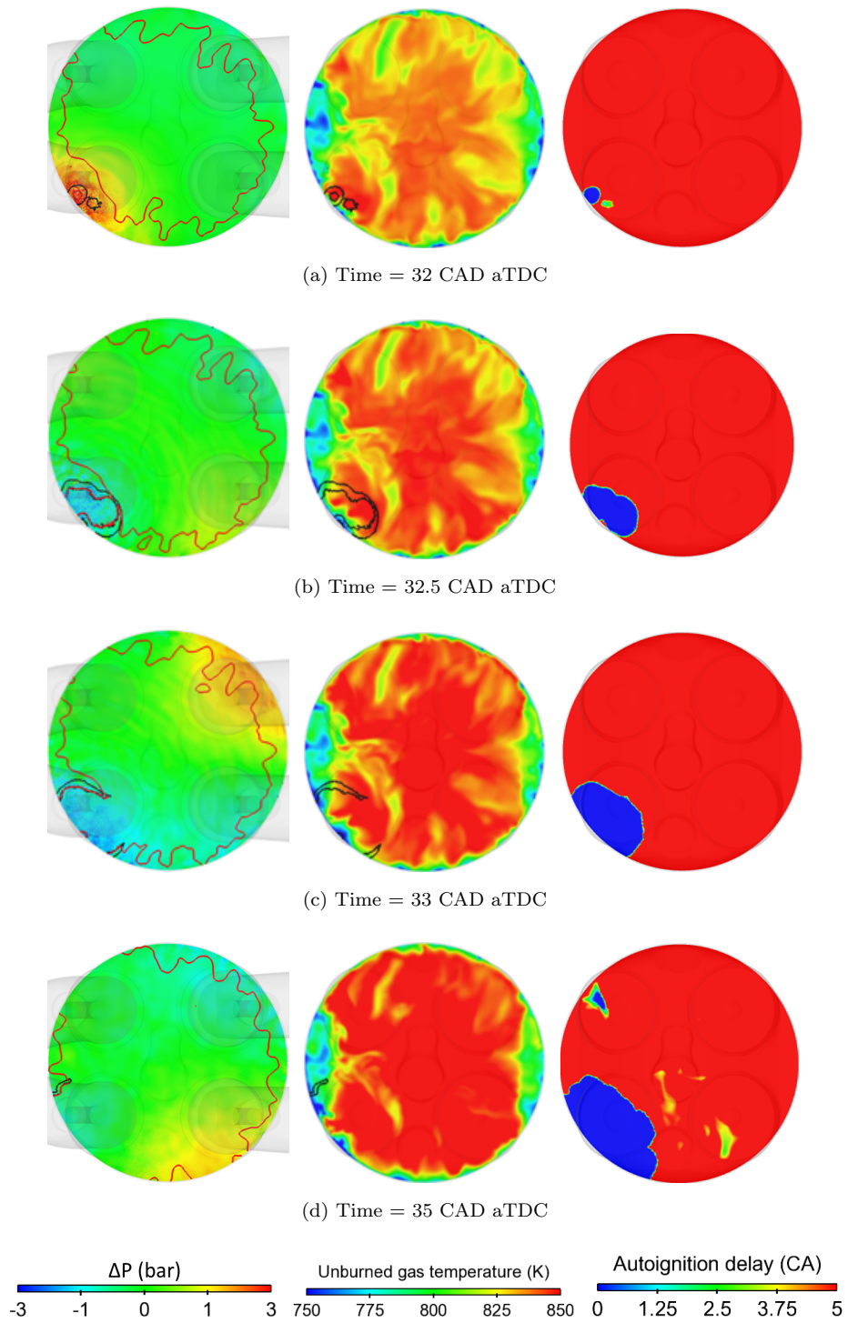
Figure 8: \Delta P evolution (left), fresh gases temperature (middle) and autoignition delay (right) at several instants for cycle 6 at ST = 8 CAD aTDC (Red line: isoline of c_\Sigma ; Black line: isoline of c_{ai} ).
