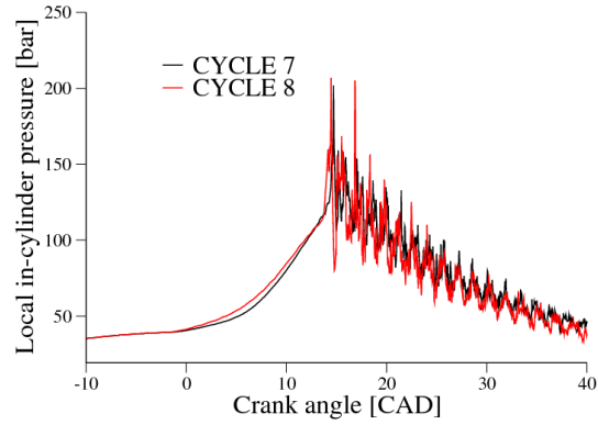
(b) Local in-cylinder pressure over CAD
