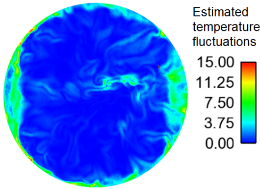
(b) Estimated temperature fluctuations [22]
