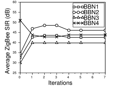
Fig 2: ZigBee SIR dynamics.
