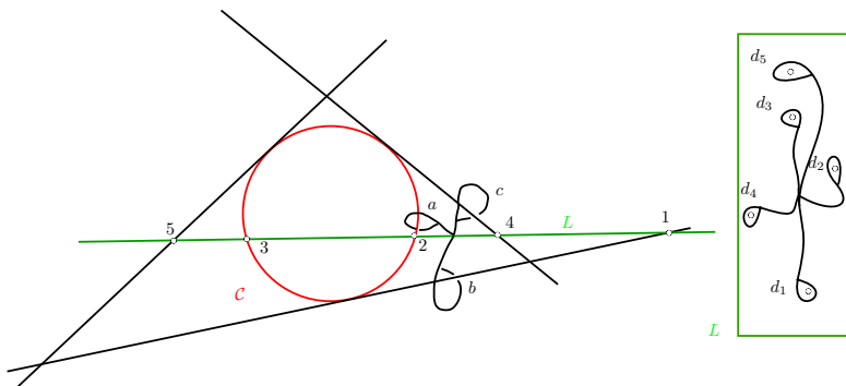
FIGURE 1. Fundamental group of the complement of the quintic \mathcal{Q} in \mathbb{P}^2 and restriction to a generic line.
