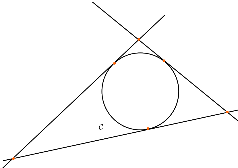
FIGURE 3. Singular locus for the foliation \mathcal{F} .
