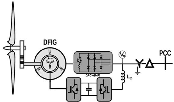
Fig. 7. Stator-side crowbar.
