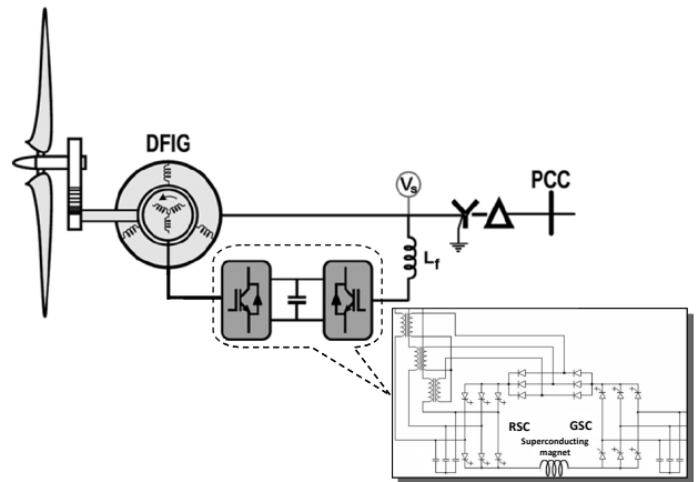
Fig. 11. DFIG-based WT equipped with a superconducting fault-current limiter.
