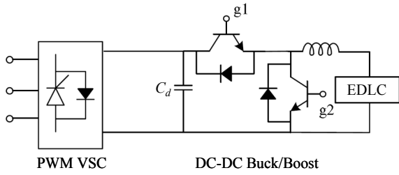
Fig. 9. ECS configuration.
