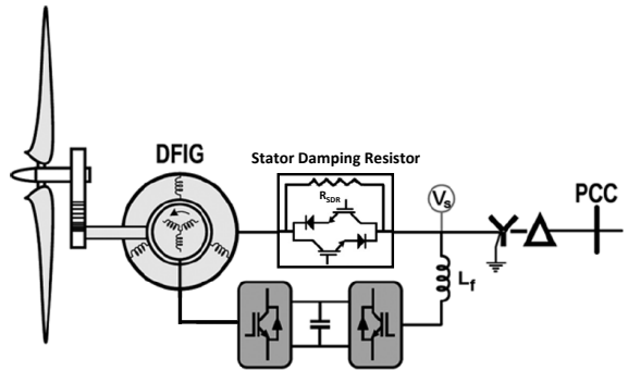
Fig. 8. DFIG-based wind turbine with SDR [28].
