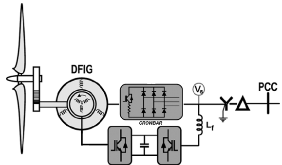
Fig. 7. Stator-side crowbar.
