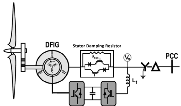
Fig. 8. DFIG-based wind turbine with SDR [28].
