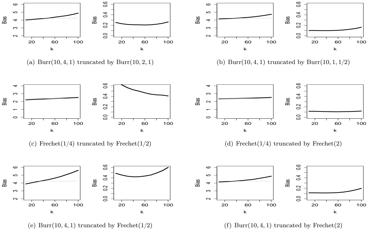
Figure 2: Bias and RMSE (respectively left and right in each subfigure) for \hat{x}_{p_n, t_n} where \gamma_1 = 1/4 , \gamma_2 = 1/2 and \alpha = 2/3 (important truncation) for subfigures (a),(c),(e), and where \gamma_1 = 1/4 , \gamma_2 = 2 and \alpha = 8/9 (mild truncation) for subfigures (b),(d),(f)
