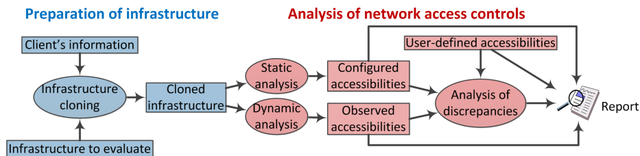
Fig. 1. Overall process
