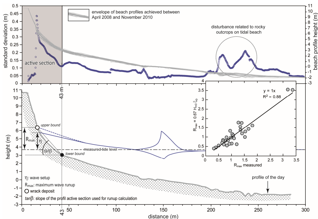
Figure 1. Method used by Cariolet and Suanéz [33] to calculate beach slope for the runup calculation. The lower bound corresponds to the limit of the profile section where changes of elevation are the most significant. This section concerns the upper part of the profile, and it is called “active section”. This limit of 43 m has been defined by calculating the standard deviation of height changes of the beach profiles (gray lines) measured between April 2008 and November 2010 (see Table 1). The upper bound corresponds to field measurements of the swash height given by the water mark limit or wrack line deposit.
