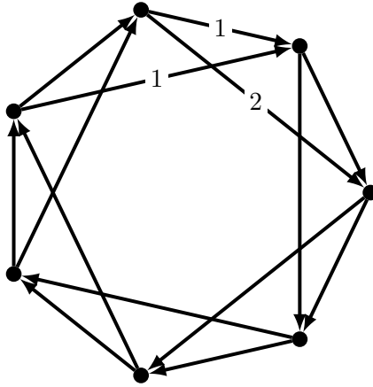
Figure 1: Illustration of the argument why \overrightarrow{C_7^2} admits no sum-colouring 2-arc-weighting. Having a weight (here, 1) on some arc (here, the topmost arc) forces two incident arcs to be weighted differently.
