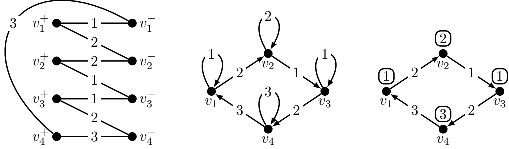
Figure 2: A digraph D (right), the same digraph D' with a loop at every vertex (middle), and the bipartite matched-representation G(D) of D (left). From a sum-colouring edge-weighting of G(D) , one can deduce a sum-colouring arc-weighting of D' , from which is deduced a sum-colouring total-weighting of D .
