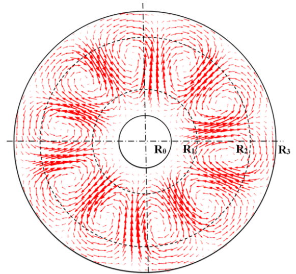
Fig. 8. Eddy-current density distribution in the middle of the copper at 1000 rpm obtained by 3-D FEM (shown as arrows).
