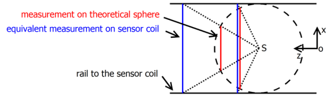
Fig. 2. Transition from sphere to the cylinder.
