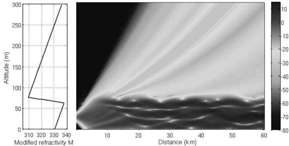
Figure A2. (left) The modified refractivity with respect to the altitude for a trilinear duct as close as possible to the arc-tangent-shaped duct from the Figure A1. (right) The 2-D associated propagation factor with respect to the distance and altitude.
