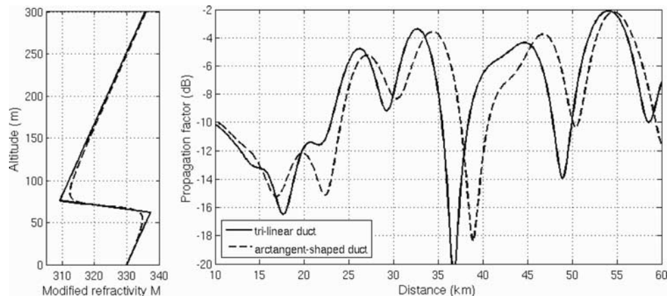
Figure A3. (left) The modified refractivity with respect to the altitude for the trilinear duct (continuous line) and for the arctangent-shaped duct (dotted line) from the Figures A1 and A2. (right) The associated propagation factors at sea level with respect to the distance.
