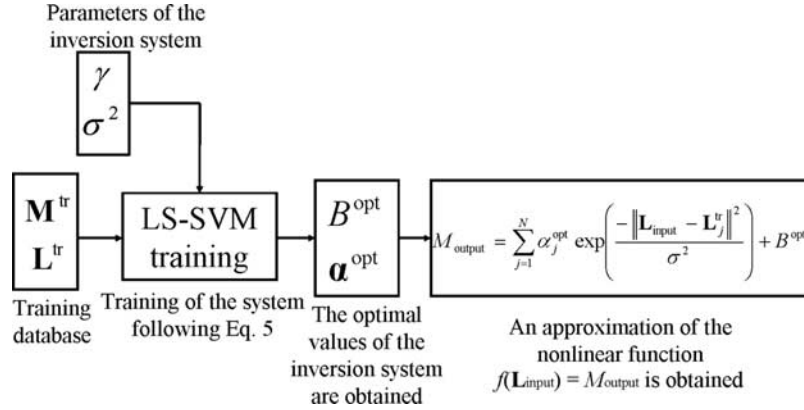
Figure 7. Scheme of the training process of LS-SVM algorithm.
