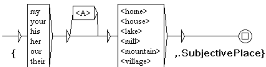
Figure 1. In Unix's syntax, the symbol \langle A \rangle represents any adjective. For example, this pattern identifies the sequences: our first home and my mill (which are considered as subjective places) and replaces them with the tagged sequences: \{our\ first\ home, SubjectivePlace\} and \{my\ mill, SubjectivePlace\} .
