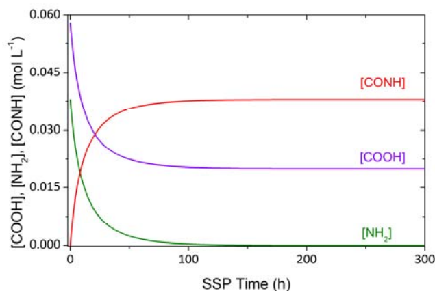
Figure 7. Simulation of PA11 SSP at 150 °C (N 2 ): simulation of and the consumption of carboxylic acids [COOH] and amine [NH 2 ] and amide build up [CONH].
