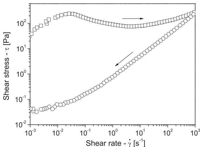
FIG. 1. Shear stress vs shear rate during a sweep test with a waxy crude oil after static cooling from 60 °C to 4 °C at -1\text{ }^{\circ}\text{C}/\text{min} and holding at 4 °C for 20 min. The up and down ramps were performed in 5 min each with a logarithmic variation [source: Mendes et al. (2014)].
