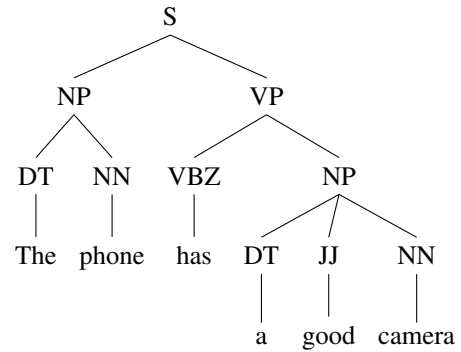
Fig. 7. Parse Tree of "The phone has a good camera"
