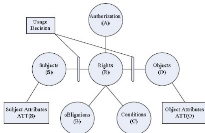
Figure 1: UCON decision model. [Zha06]
