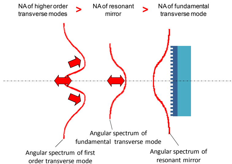
Fig. 1. Sketch of a laser grating-mirror with 1D representation of the angular width \Delta\Phi_0 of the fundamental and higher order transverse mode \Delta\Phi_1 relative to that of the resonant mirror for the filtering out of the high order transverse modes.
