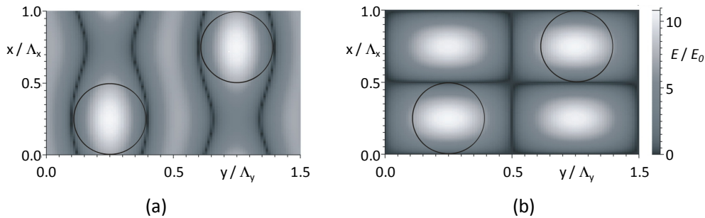
Fig. 10. \text{TE}_0 modal electric field modulus distribution over one period in the \text{Si}_3\text{N}_4 waveguide of the element of Fig. 9 at resonance under normal incidence of a x-polarized wave. The black circles indicate the position of the holes at the upper surface of the cover layer. (a) Modulus of the x component of the electric field, (b) of its y component.
