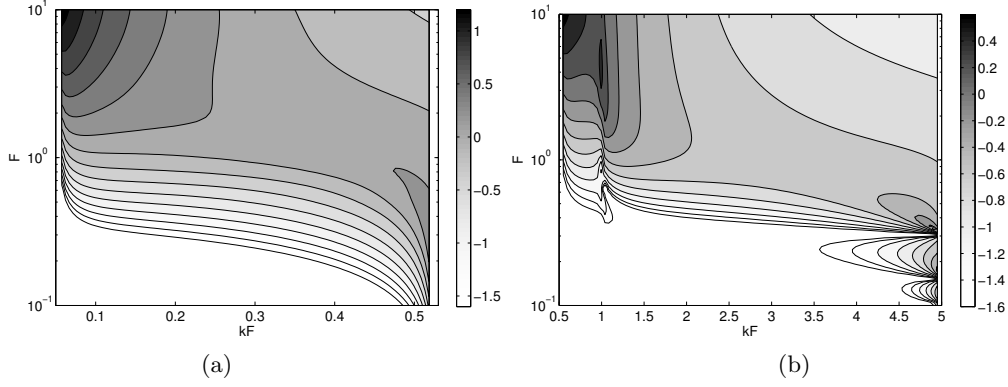
FIGURE 9. Contour levels of the function \log_{10} V in the (kF, F) plane for U_0 = 0.1 and (a) \alpha = \pi/60 or (b) \alpha = \pi/6 . The function V is defined for \sin \alpha < kF < \sin \alpha / U_0 only (condition of existence of a critical point).
