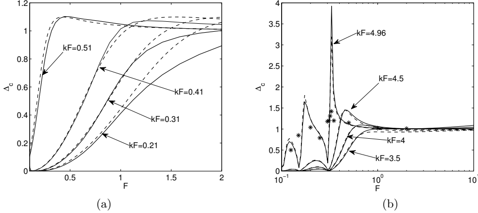
FIGURE 11. The function \Delta_c versus F for different values of kF for (a) \alpha = \pi/60 and (b) \alpha = \pi/6 . Solid lines: numerically computed values; Dashed lines: expression (3.19a,b). The stars in (b) are estimates obtained from the direct numerical simulation for kF = 4.96 , Re = 593 and h = 0.12 .
