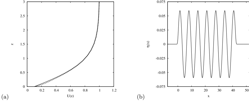
FIGURE 2. Inlet (solid line) and at the summit of an oscillation x = 30.3 (dashed line) velocity profiles (a) at Re = 593 and h = 0.06 . Graph of the lower boundary \eta(x) (b) of the small computational domain at h = 0.06 .
