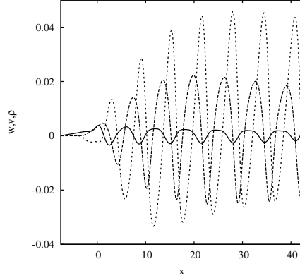
FIGURE 4. Streamwise profile of the normal velocity w (solid line), transverse velocity v (dashed line) and density \rho (dotted line) at z_c = 0.75 . Re = 593 , F = 1.046 , k = 1.041 , \alpha = \pi/4 and h = 0.06
