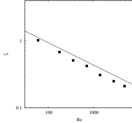
FIGURE 8. Thickness of the critical layer as a function of the Reynolds number measured on the lee side of a hill at x = 7.5\pi/k . The theoretical prediction (solid line) is compared to the numerical simulations (■). h = 0.03 , F = 1.046 , k = 1.041 and \alpha = \pi/4 .
