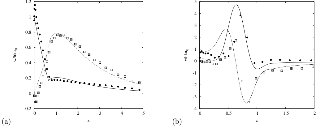
FIGURE 6. Normal profile of (a) normal velocity w and (b) transverse velocity v . The profiles are measured on the lee side of the undulations at x = 7\pi/k ( \bullet , solid line) and on the bottom of the undulation at x = 7.5\pi/k ( \square , dashed line). Symbols correspond to numerical simulations and lines to theoretical predictions. h = 0.03 , F = 1.046 , k = 1.041 , Re = 1423 and \alpha = \pi/4 .
