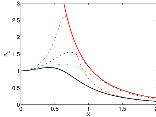
FIGURE 12. Function \Delta_c = |\tilde{w}(\tilde{z}_c)/\tilde{w}(0)| versus X . The solid black line is \Delta_c^-(X) , that is for kF < 1 . The solid red line is \Delta_c^+_{\max}(X) (maximum value of \Delta_c^+ over all \Phi for kF > 1 ). The dotted lines are \Delta_c^+ for \Phi = \pi/2 (green), \Phi = 2\pi/3 (blue) and \Phi = 5\pi/6 (red).
