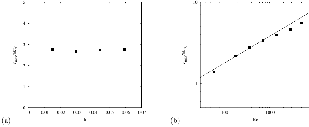
FIGURE 7. Renormalised amplitude of the critical layer v_{\max}/(hkU_0) as a function of (a) the height of the hills h and (b) the Reynolds number. Numerical values (■) obtained at x = 7.5\pi/k are compared with the theoretical prediction (solid line) given by (3.14). F = 1.046 , k = 1.041 and \alpha = \pi/4 . In (a) Re = 593 and in (b) h = 0.03 .
