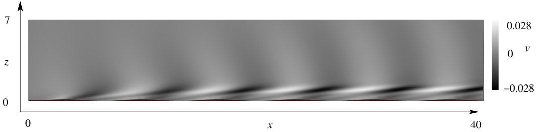
FIGURE 3. 2D field of the transverse velocity v(x, z) for h = 0.06 , F = 1.046 , k = 1.041 , Re = 1186 and \alpha = \pi/4 .
