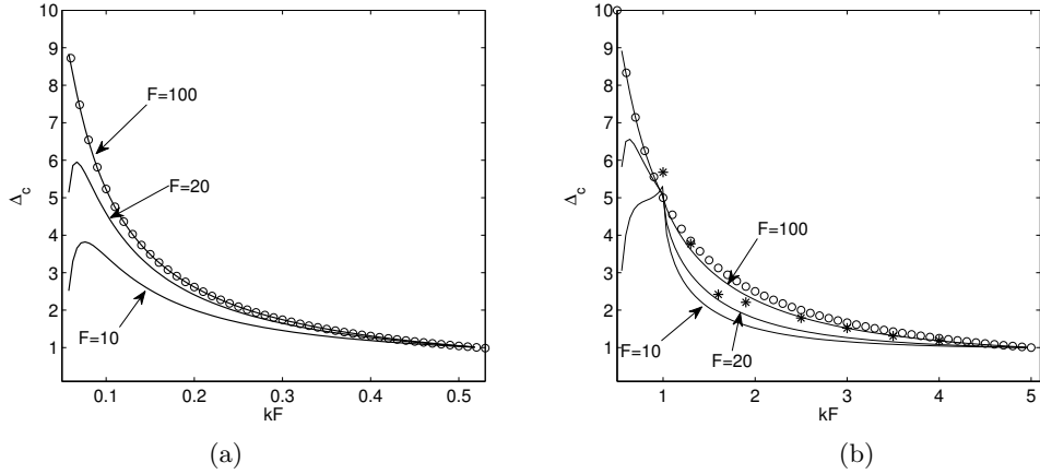
FIGURE 10. The function \Delta_c versus kF for different values of F for (a) \alpha = \pi/60 and (b) \alpha = \pi/6 . Solid lines: numerically computed values; Symbols: expression (3.17). The stars in (b) are estimates obtained from the direct numerical simulation for F = 10 , Re = 593 and h = 0.12 .
