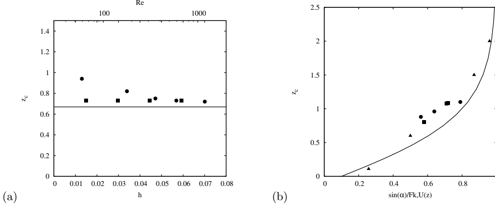
FIGURE 5. Position of the critical layer z_c measured at the maximum of v . In (a), z_c is plotted as a function of h (■) and as a function of Re (●) for F = 1.046 , \alpha = \pi/4 and k = 1.041 . In (b), z_c is plotted as a function of \sin \alpha/kF for Re = 593 and h = 0.06 . In (b), symbols correspond to variations of F (■), k (●) and \alpha (▲) and the solid line corresponds to the velocity profile U(z) .
