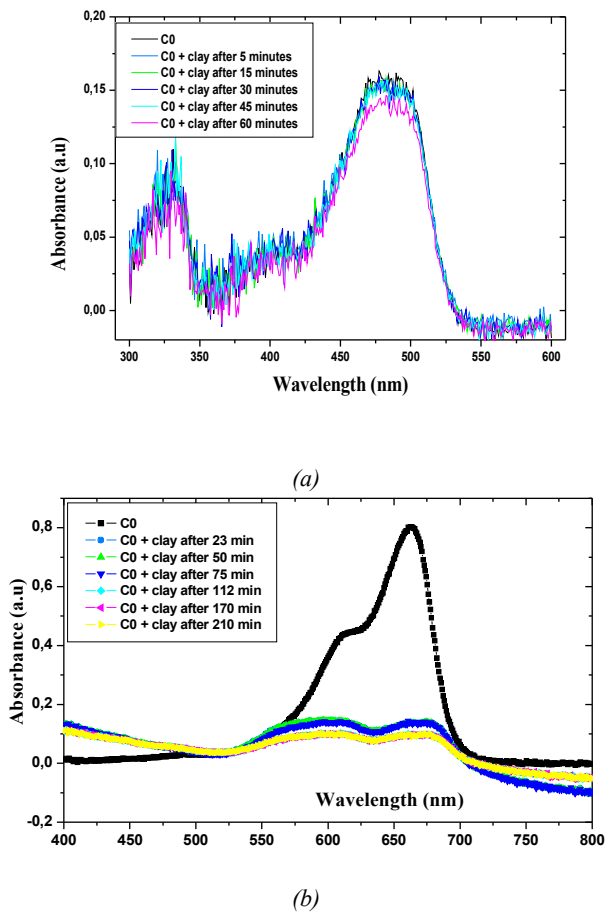
Fig. 2. UV absorption spectra of orange G (a) and methylene blue (b) versus adsorption time onto stevensite.
