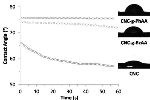
Figure 10. Contact angle measurements of neat CNC (O) and functionalized with PhAA (◇) and BzAA (x).
