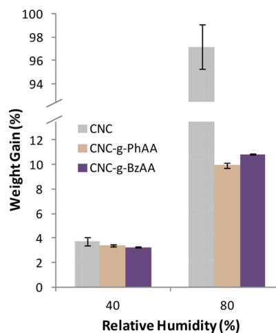
Figure 11. Water vapor adsorption of modified and unmodified CNC placed at 40 and 80% of RH.
