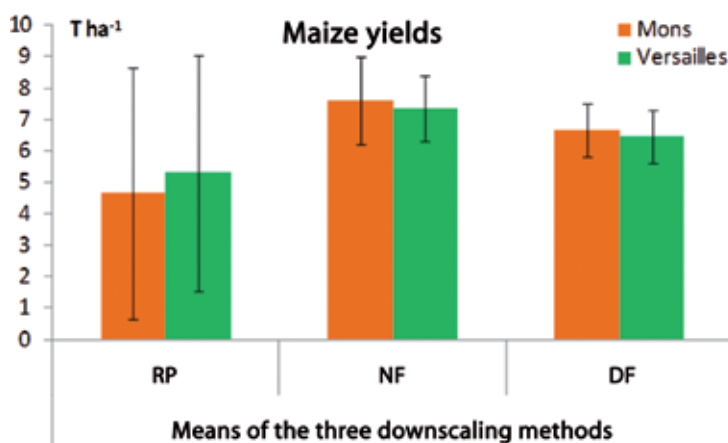
Figure 8: change in grain maize yields (variety Mérihel, soil 1) between the three periods with an indication of the variability*, combining the year-to-year variability with that due to the climate downscaling methods.
