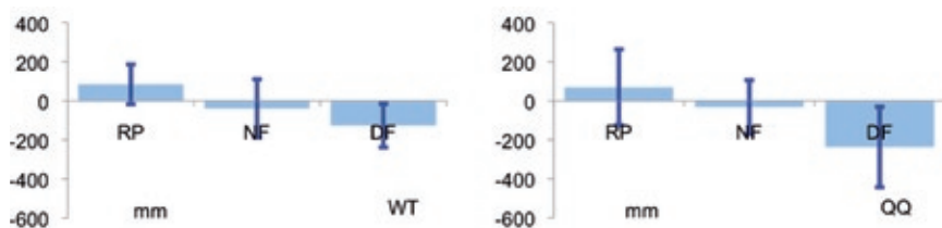
Figure 2: annual climatic water deficit (rainfall-ET 0 ) in the RP, the NF and the DF at Rennes. ARPÈGE, A1B. Downscaling methods: WT (left) and QQ (right). The ET 0 is calculated without correcting for the CO 2 (cf. MODELS section).
