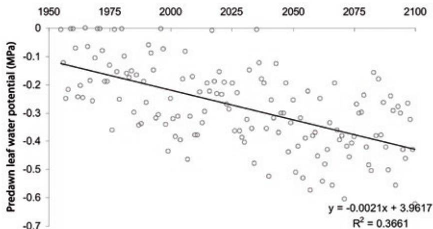
Figure 5: worsening trend in the annual water deficit at Clermont-Theix for tall fescue with the A1B scenario and the WT downscaling method The basic leaf water potential measures the water stress “experienced” by the vegetation.
