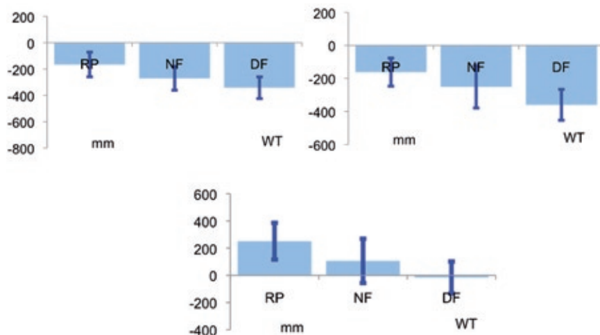
Figure 2: annual climatic water deficit (rainfall-ET 0 ) in the RP, NF and DF at Colmar (top left), Dijon (top right) and Mirecourt (bottom). ARPÈGE A1B. WT downscaling method. The ET 0 is calculated without correcting for the CO 2 (cf. MODELS section).
