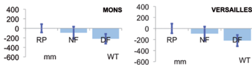
Figure 2: annual climatic water deficit (rainfall – ET_0 ) in the RP, the NF and the DF at Mons (left) and at Versailles (right). ARPEGE AIB. WT downscaling method. The ET_0 was calculated without the correction for CO_2 (cf. MODELS section).
