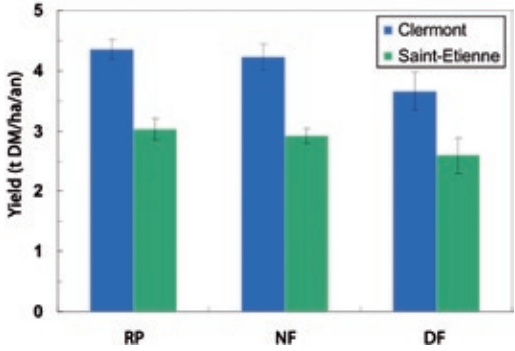
Figure 12: change in yield of pines (45-year rotation, soil 3, WT downscaling method) between the three periods, with the year-to-year variability.
