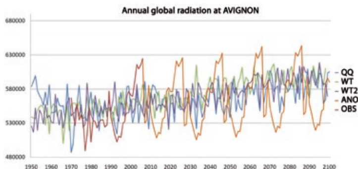
Figure 3: change in total annual global radiation (J/cm 2 /yr) from 1950 to 2100 at Avignon. ARPÈGE A1B. Standard downscaling methods: ANO, WT and QQ, to which were added the WT2 method (cf. CLIMATE) and the data observed on the RP.
