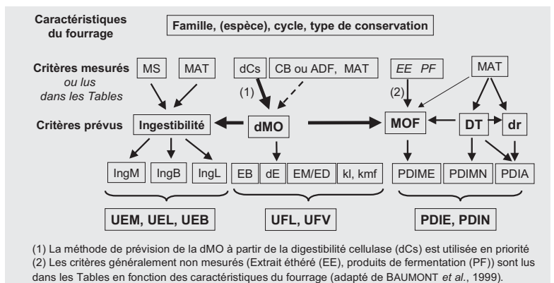
FIGURE 2 : Arrangement of the calculations for the forecast of the feeding value of a forage .
