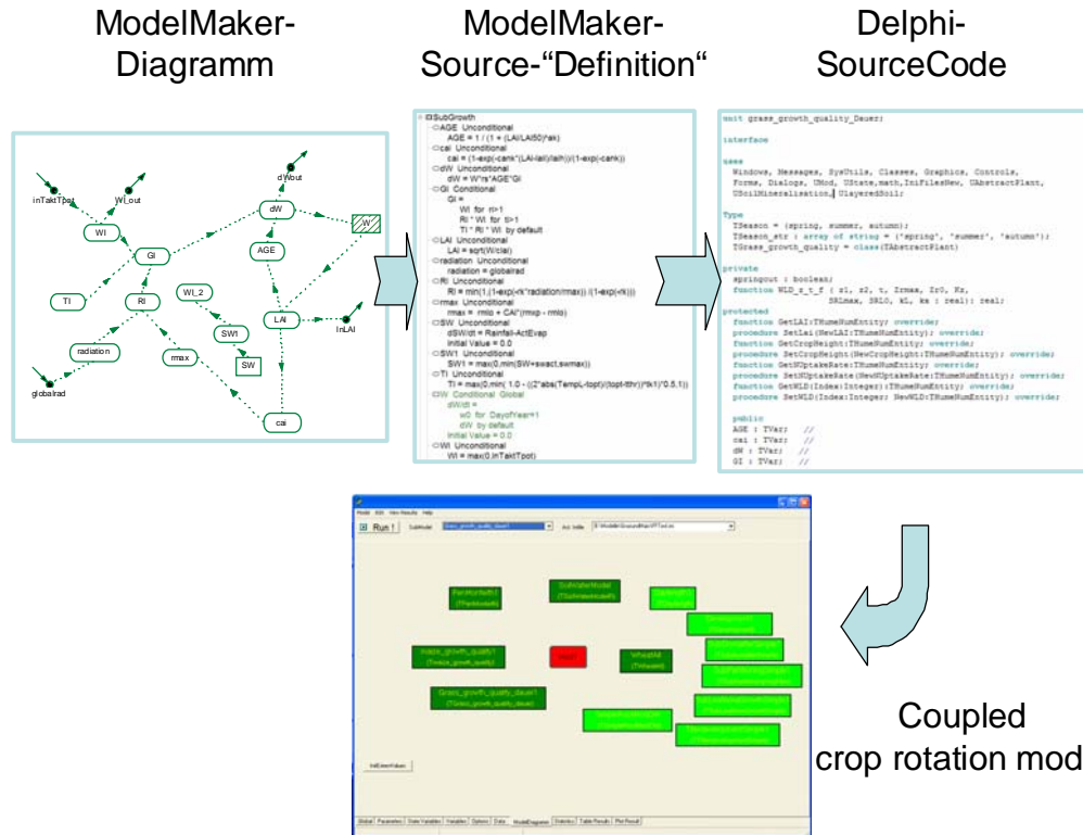
Fig. 1: Example for integration an existing submodel (here a simple crop simulator for DM production of rye grass) into a larger crop rotation model.
