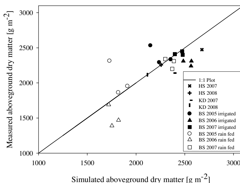
Fig. 1: 1:1 plot of measured and simulated aboveground dry matter yield [g m -2 ]. Data set of 3 different sites (HS, KD and BS) out of 4 years (2005-08). For BS irrigated and rain fed variants are shown, same symbols hide different hybrids. RMSE: 237 \text{ g m}^{-2} .
