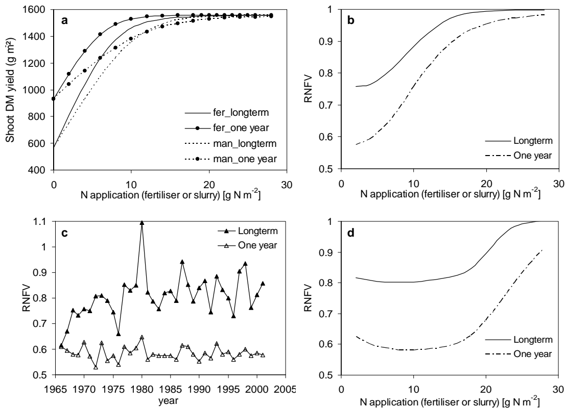
Fig. 1. Simulation results, provided as (a) maize shoot dry matter yield (g m -2 y -1 ); (b) relative N fertilizer value (RNFV) of manure with respect to dry matter yield; (c) RNFV of manure with respect to N yield, time trend with 12 \text{ g N m}^{-2} \text{ y}^{-1} (d) RNFV of manure with respect to N yield. (a), (b) and (d) are averages of 36 years.
