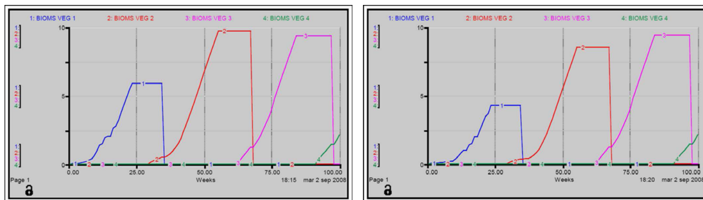
Figure 1: Growth simulation of bananas on bare soil (on the left) and with grass cover (right)
