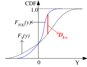
Fig. 1 Difference of F_{Y|X_i}(y) and F_Y(y) is measured by D_{k-s} .
