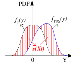
Fig. 1 Shift of f_{Y|X_i}(y) from f_Y(y) is measured by s_{X_i} .
