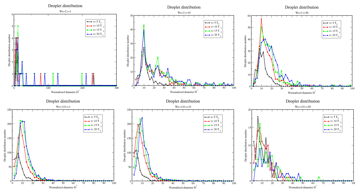
Figure 3. Probability density functions (PDF) of droplet size for We=2 (top line) and We=110 (bottom column). From left to right, \rho_2/\rho_1=1, 10 and 50 . Time 5 T_0 (black line), 10 T_0 (red line), 15 T_0 (green line) and 20 T_0 (blue line) are plotted.
