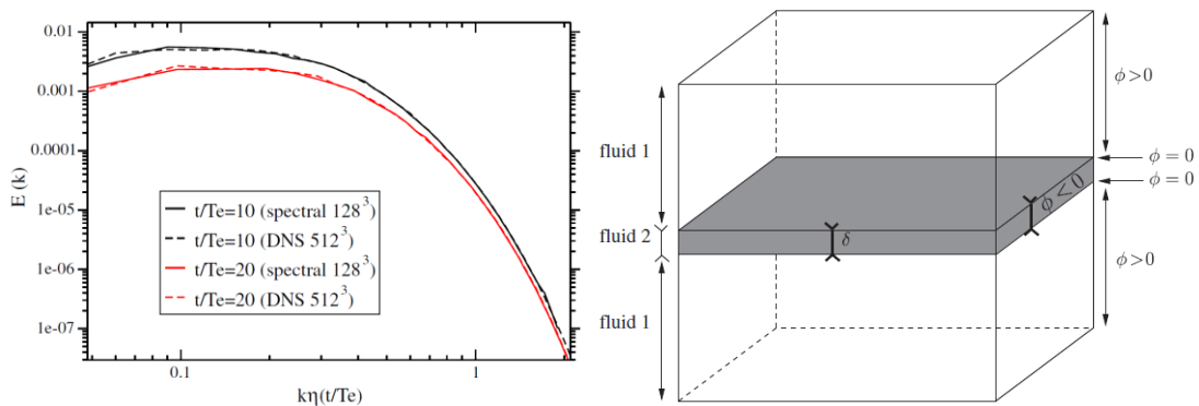
Figure 1. Initial energy density spectrum of the HIT field (left) and initial position of the liquid sheet (fluid 2, right).
