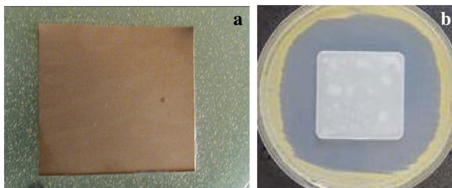
Fig. 6. Diffusion test showing that (a) no inhibition zone is observed around a 25 × 25 mm 2 TiO 2 -Cu sample whereas (b) there is such inhibition zone (gray area) around a reference sample consisting of a piece of plastic treated with triclosan as antibacterial agent.
