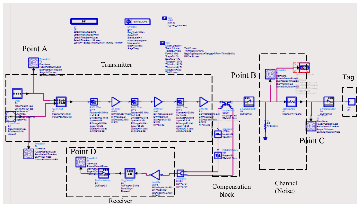
Fig1: block diagram of the RFID communication system
