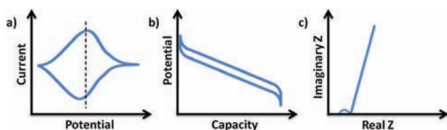
Fig. 8 The general electrochemical features of pseudocapacitive materials. (a) In a cyclic voltammetry experiment, the shape is rectangular and if peaks are present, they are broad and exhibit a small peak-to-peak voltage separation. (b) In a galvanostatic experiment, the shape is sloping so that a capacitance value, \Delta Q/\Delta E , may be assigned at each point, and the voltage hysteresis is small. Here, Q is the capacity and E is the potential window. (c) In an AC impedance experiment, the Nyquist representation will contain a vertical line with a phase angle of 90^\circ or less. A semi-circle at high frequencies, associated with charge-transfer resistance, may also be present.
