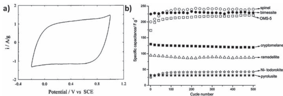
Fig. 11 (a) CV at 5 \text{ mV s}^{-1} of a thick composite electrode of amorphous \text{MnO}_2 \cdot n\text{H}_2\text{O} in 2 \text{ M KCl} electrolyte. At this sweep rate, the capacitance was \sim 200 \text{ F g}^{-1} . Reprinted from ref. 48, with permission from Elsevier. (b) The specific capacitance and cyclability of different \text{MnO}_2 allotropes under investigation for high-rate energy storage as tested in a composite electrode architecture in 0.5 \text{ M K}_2\text{SO}_4 electrolyte at 5 \text{ mV s}^{-1} . Reprinted with permission from ref. 50. Copyright 2009 American Chemical Society.
