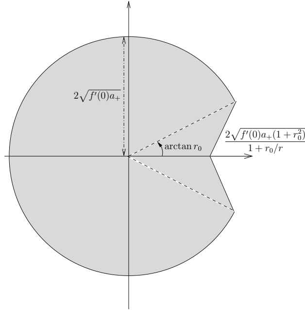
Figure 4: The non-convex expansion set \bar{\mathcal{S}} = \underline{\mathcal{S}} given by Proposition 3.13.
