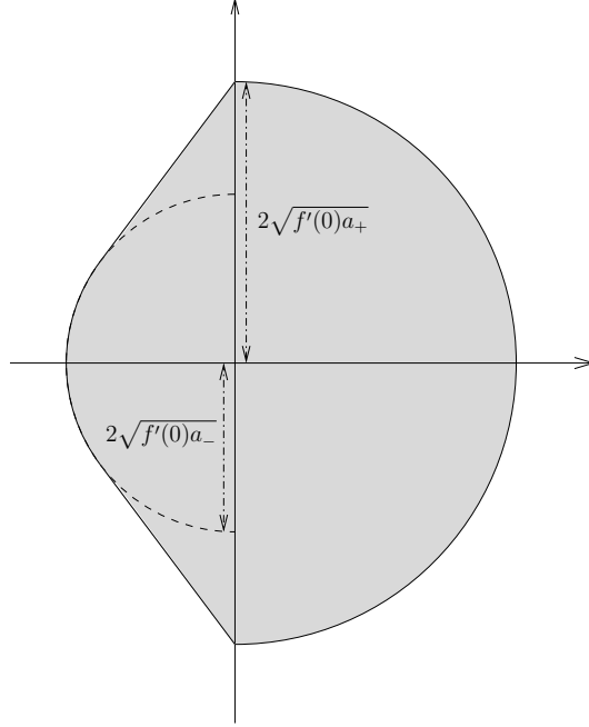
Figure 3: The expansion set \overline{\mathcal{S}} = \underline{\mathcal{S}} given by Proposition 3.11 for N = 2 .
