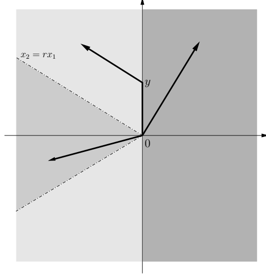
Figure 6: This figure represents the geodesics of the minimization problem (107). The darker area corresponds to the case x_1 > 0 and the lighter one to the case x_1 < 0 and |x_1| \geq r|x_2| . The large arrows represent the ray paths in each of these areas.
