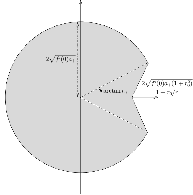
Figure 3: The non-convex expansion set \bar{\mathcal{S}} = \underline{\mathcal{S}} given by Proposition 2.10.
