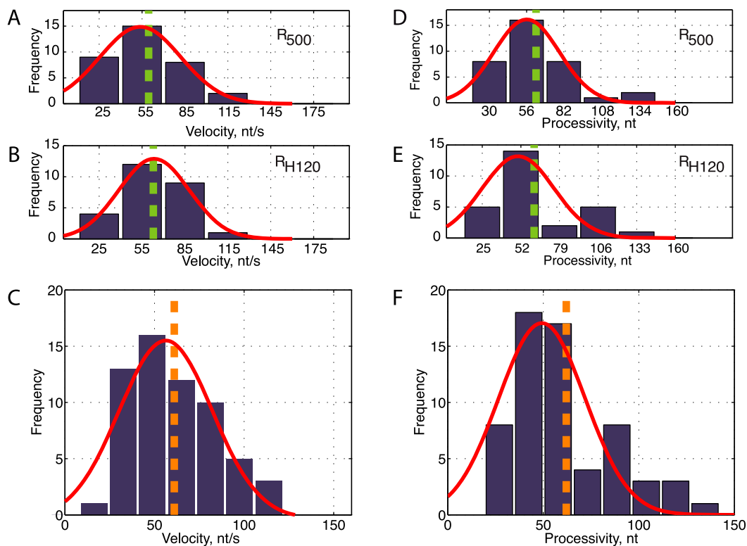
Figure 4. Rates and processivities of Rho translocation on single-stranded RNA. (A and B) Histograms of velocities of Rho translocation on R_{500} (panel A) and R_{H120} (panel B). Gaussian fits are represented in red (mean \pm SEM: 50 \pm 4 nt/s for R_{500} and 56 \pm 4 nt/s for R_{H120} ), dashed green lines show unweighted averages ( 59.6 \pm 4 nt/s for R_{500} and 62.8 \pm 4 nt/s for R_{H120} ). (C) Histogram of compiled Rho single-molecule velocities (blue bars) fit to a Gaussian function (red line) indicates a mean rate of 56 \pm 3 nt/s (mean \pm SEM). Average velocity of 61 \pm 3 nt/s (mean \pm SEM) is indicated with a vertical dashed line. N = 62 . (D and E) Histogram of Rho translocation processivities on R_{500} (panel A) and R_{H120} (panel B). Gaussian fits are represented in red (mean 56 \pm 4 nt for R_{500} and 48 \pm 4 nt for R_{H120} ), dashed green lines show the unweighted averages of all measurements ( 62 \pm 4 nt for R_{500} and 61 \pm 4 nt for R_{H120} ). (F) Histogram of compiled Rho single-molecule processivities (blue bars) fit to a Gaussian function (red line) showing a maximum at 49 \pm 3 nt (mean \pm SEM). Average processivity 62 \pm 3 nt (mean \pm SEM) is indicated with a vertical dashed line. Only events with processivities twice larger than the instrument noise ( \sim 10 nm SD) were considered. N = 62 .
