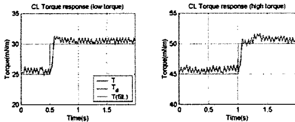
Fig. 6: Closed loop Step Response Using a Non-Linear PI Controller
