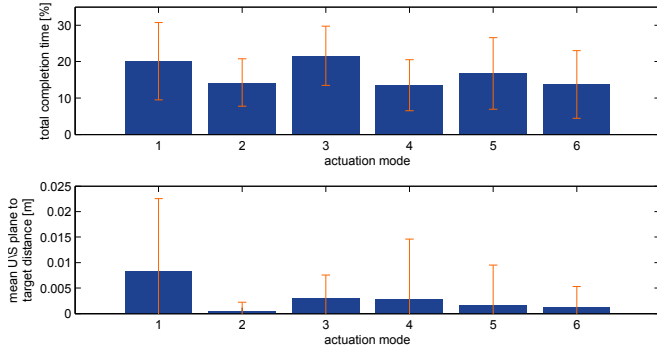
Fig. 4. Results of tests 1: mean localization time and U/S-plane to target distance.
