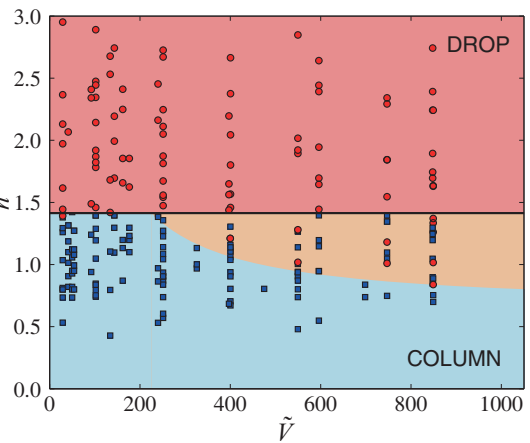
Figure 6: Morphology diagram in the parameter space (\tilde{V}, \tilde{h}) using silicone oil ( \theta_E = 0^\circ ) on parallel fibers ( \delta = 0^\circ ) of radii a = [100, 150, 230] \mu\text{m} and a volume of liquid V \in [0.5, 4] \mu\text{l} . Red circles show the drop morphology and blue squares the column morphology. The light orange region corresponds to the region where both morphologies are observed. The horizontal solid line corresponds to the theoretical maximum separation distance where the column state is possible, \tilde{d}_{max} = \sqrt{2} .
