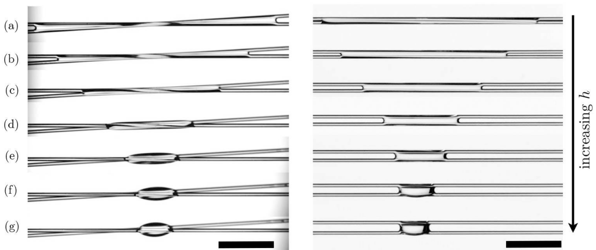
Figure 4: Evolution of the morphology of a drop of volume V = 2 \mu\text{l} of silicone oil (5 cSt) on two non-touching crossed fibers of radius a = 150 \mu\text{m} , tilted by an angle \delta = 4^\circ as the distance h between the fibers is increased: top (left) and side (right) views. The liquid starts in a column state at small separation distances, (a) h = 0 . As the distance h is increased, the liquid adopts a drop morphology (f)-(g). Scale bars are 5 mm.
