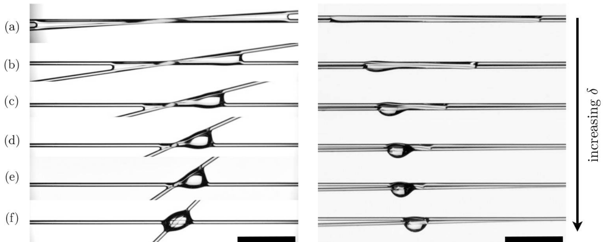
Figure 3: Evolution of the morphology of a drop of volume V = 2 \mu\text{l} of silicone oil (5 cSt) on two touching crossed fibers ( h = 0 ) of radius a = 150 \mu\text{m} as the angle \delta between the fibers is varied: top (left) and side (right) views. The liquid starts in a column state for a small tilting angle, (a) \delta = 4^\circ . As the angle is increased, a mixed morphology is observed: (b) \delta = 9^\circ , (c) \delta = 15^\circ , (d) \delta = 25^\circ and (e) \delta = 35^\circ . Finally, at larger angles, (f) \delta = 45^\circ , a drop lies at the crossing point of the fibers. Scale bars are 5 mm.
