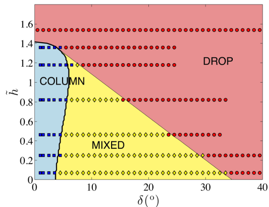
Figure 8: Morphology diagram for a drop of silicone oil places on separated crossed fibers of radii a = 150 \mu\text{m} in the parameter space (\delta, \tilde{h}) using a volume \tilde{V} = 592 of silicone oil ( \theta_E = 0^\circ ). Red circles show the drop morphology, blue squares the column morphology and yellow diamonds are the mixed morphology. The thick solid line is the prediction of our model.
