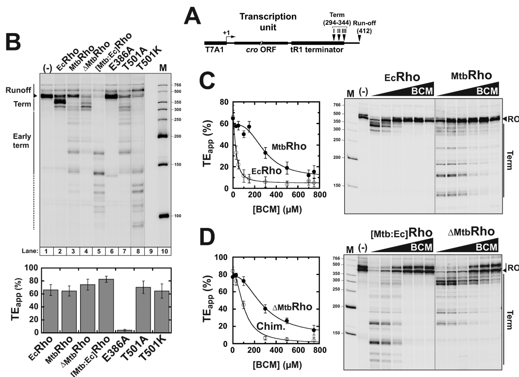
Figure 6. Transcription termination experiments. (A) Schematic of the DNA template containing the \lambda tR1 terminator used in in vitro termination experiments. (B) Both the NTD and CTD of M_{tb} Rho affect its transcription termination activity. A representative denaturing PAGE gel showing the products of transcription termination experiments performed under standard 'chase' conditions with E. coli RNAP and the \lambda tR1 terminator in the presence of various Rho factors (indicated above gel lanes). Intensity of the T501K lane had to be adjusted separately (as indicated by vertical dotted lines) because reactions with the T501K mutant consistently yielded lower product amounts. Apparent termination efficiencies ( TE_{app} ) are indicated below the gel ( N_R = 3 ). (C) A higher concentration of BCM is required to inhibit M_{tb} Rho than E_{c} Rho under standard transcription termination 'chase' conditions ( N_R = 3 ). (D) Comparison of the termination activities of the [M_{tb}:E_{c}] Rho and \Delta M_{tb} Rho variants in the presence of BCM indicates that structural components conferring BCM resistance to M_{tb} Rho are located mostly in its CTD. In the figure, the intensity and gamma settings were adjusted to facilitate the comparison of termination signals in the various gel panels (separated by dotted lines). Gel images without gamma setting adjustments are presented in Supplementary Figures S6 and S7F.
