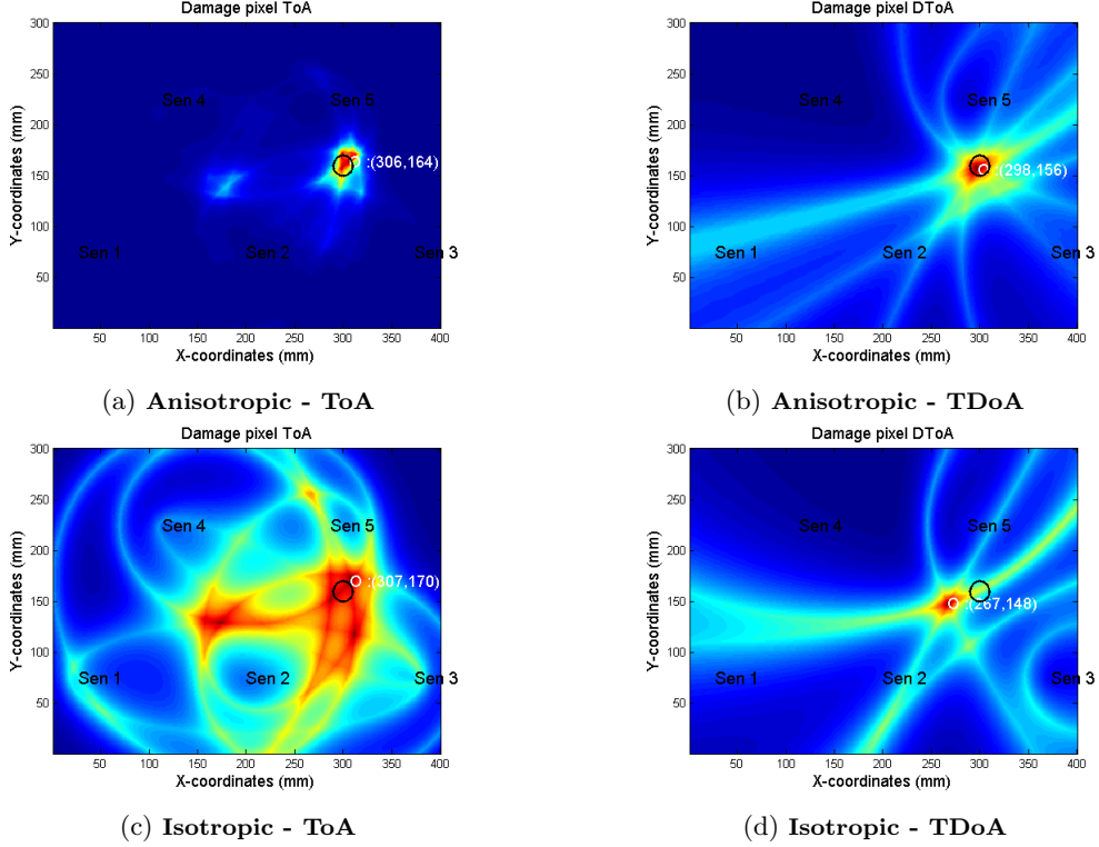
Figure 5: Damage localization results - numerical study - : (a) ellipse method using the proposed parametrized group velocity profile,(b) hyperbola method using the proposed parametrized group velocity profile, (c) ellipse method using an isotropic velocity profile, and (d) hyperbola method using an isotropic velocity profile.
