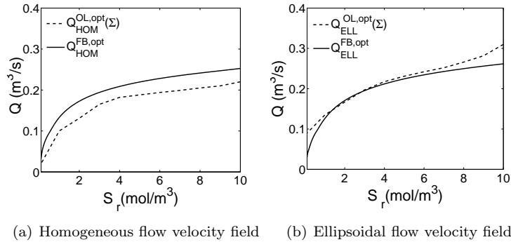
Figure 5: ODE-PDE model: Case \tau_b \approx \tau_r . Comparison between the feedback approximations Q_{\text{FB,opt}}^{\text{FB,opt}} (depicted with solid lines) and Q_{\text{OL,opt}}^{\text{OL,opt}}(\Sigma) (depicted with dashed lines).
