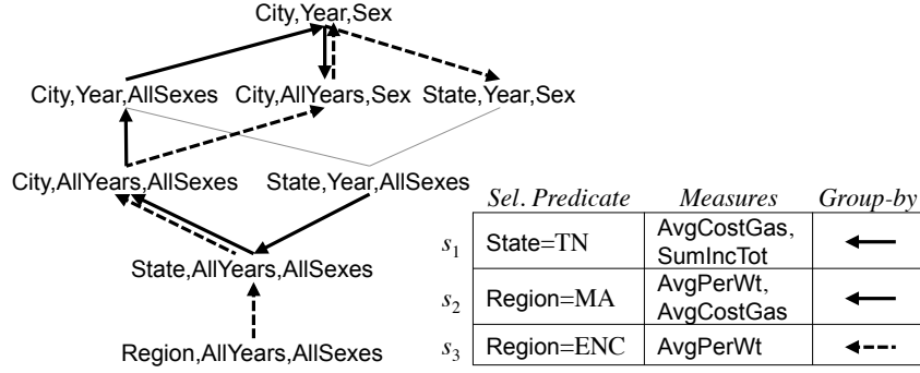
Fig. 2. A log for our working example
