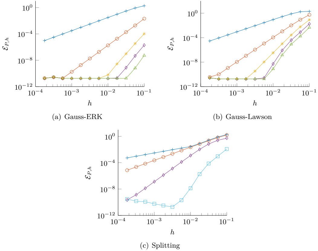
Figure 2: Evolution of \mathcal{E}_{P,h} error with respect to the time step
