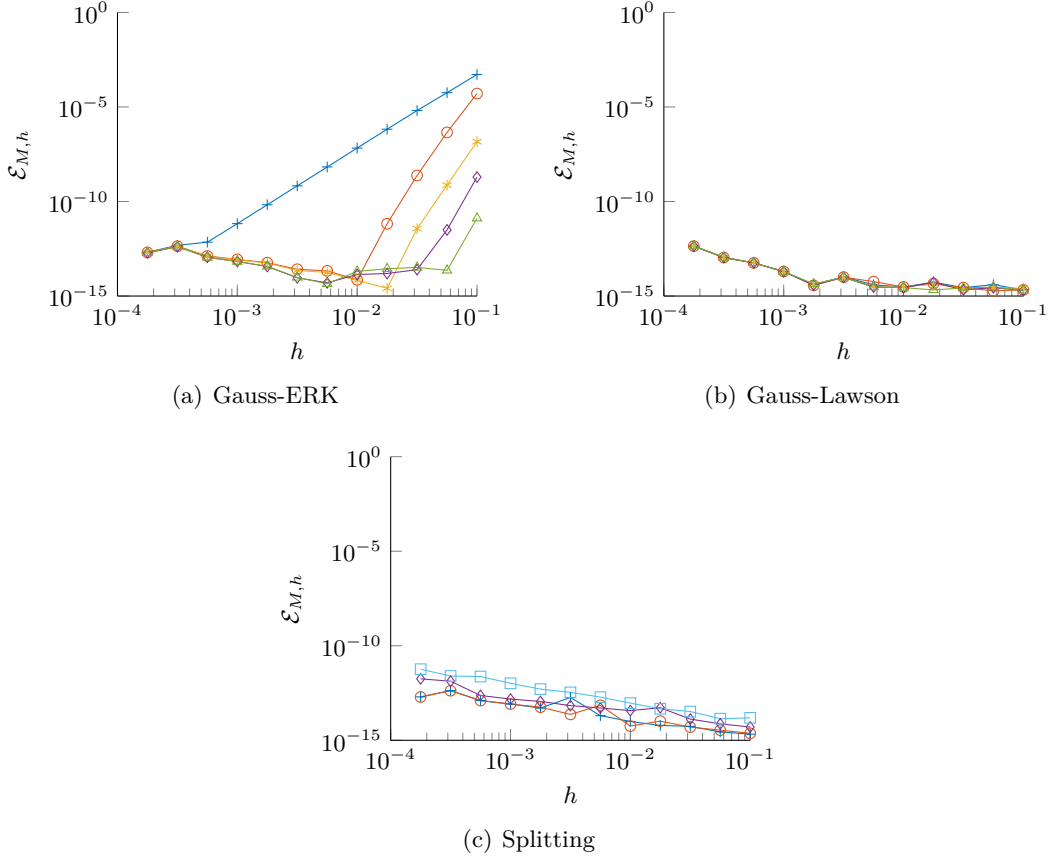
Figure 3: Evolution of \mathcal{E}_{M,h} error with respect to the time step
