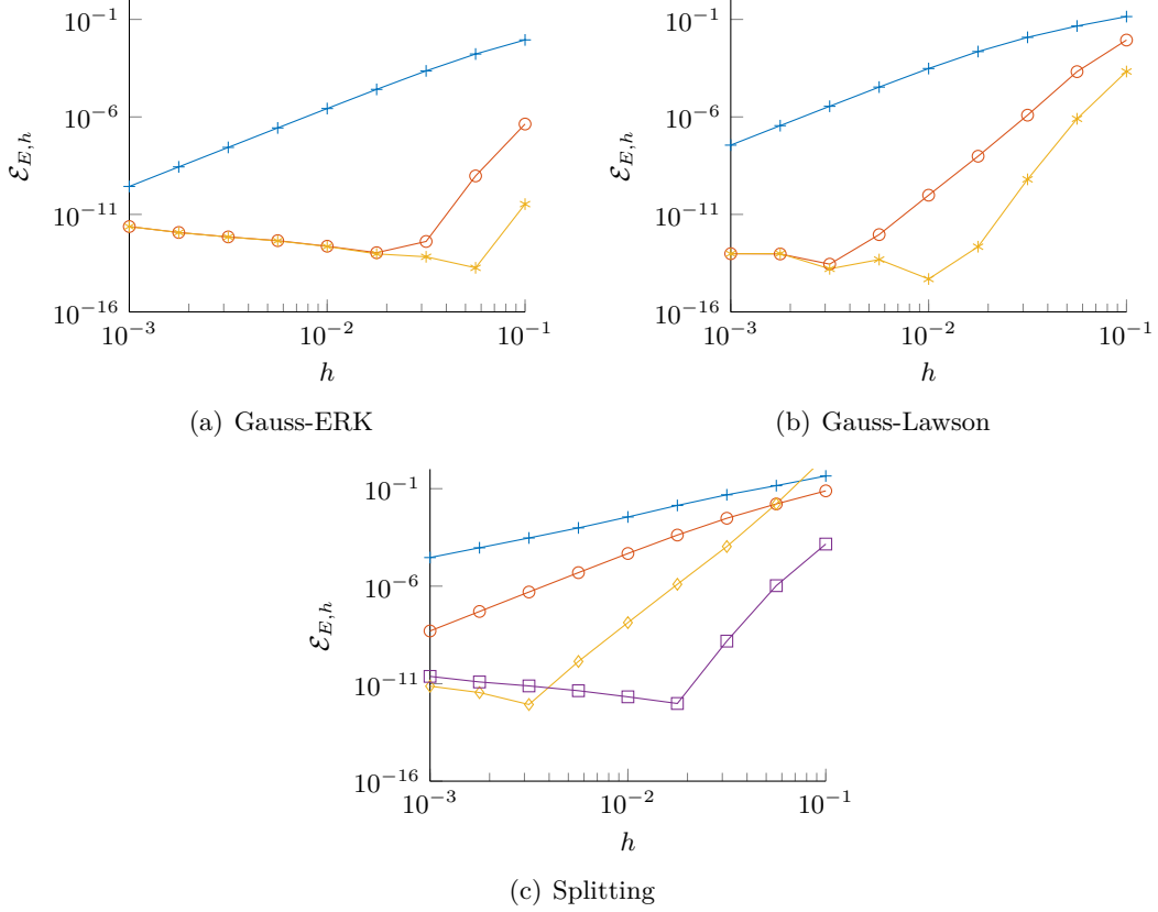
Figure 8: Evolution of \mathcal{E}_{E,h} error with respect to the time step
