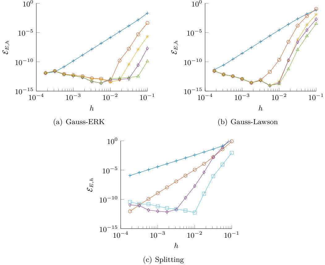
Figure 4: Evolution of \mathcal{E}_{E,h} error with respect to the time step
