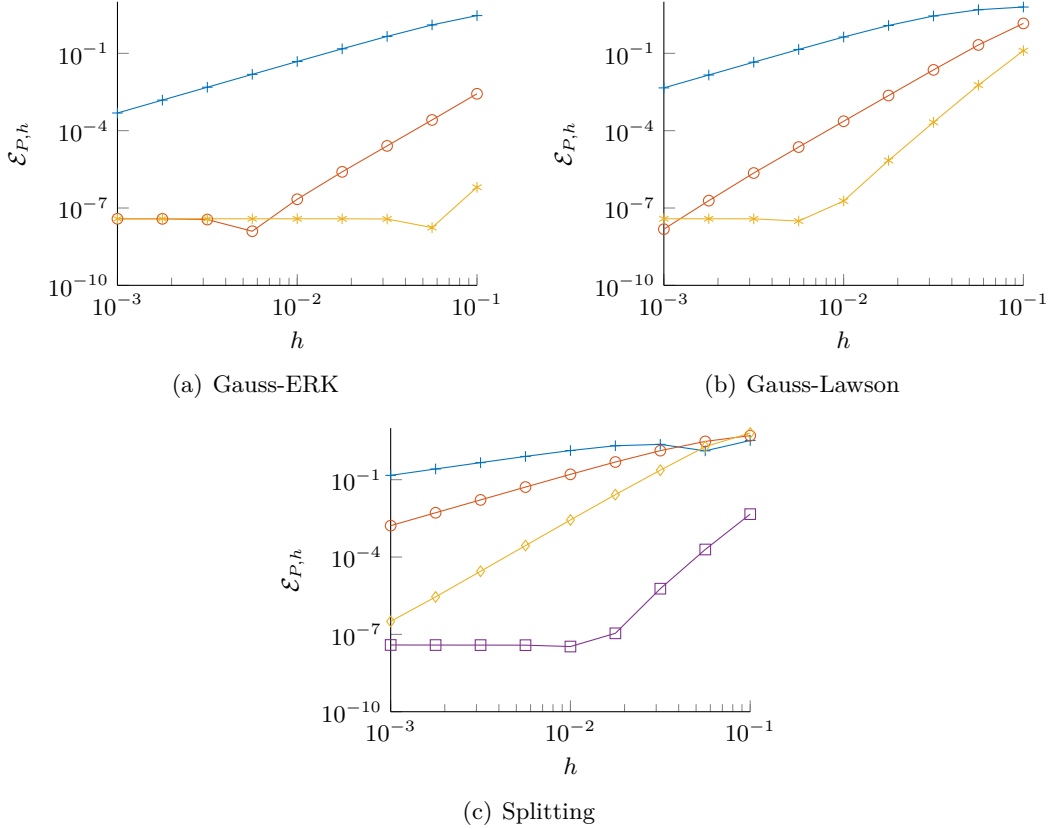
Figure 6: Evolution of \mathcal{E}_{P,h} error with respect to the time step
