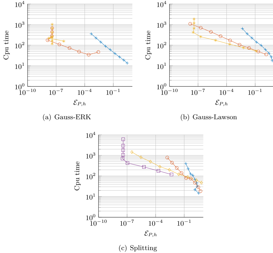
Figure 9: Evolution of the Cputime with respect to \mathcal{E}_{P,h} error
