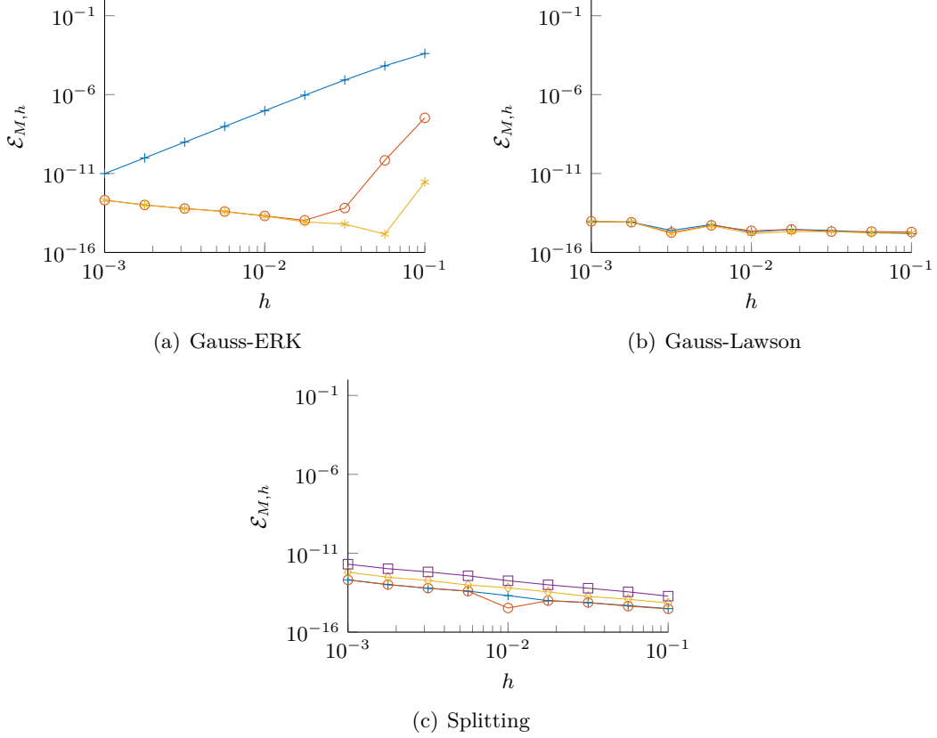
Figure 7: Evolution of \mathcal{E}_{M,h} error with respect to the time step
