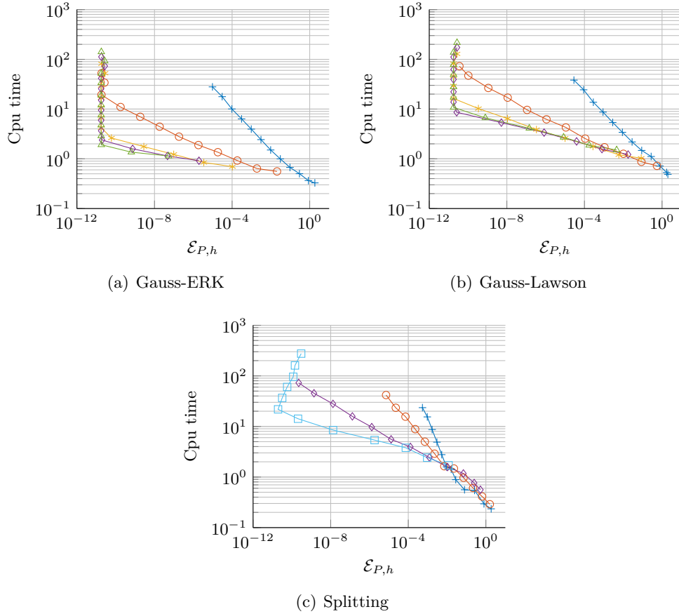
Figure 5: Evolution of the Cputime with respect to \mathcal{E}_{P,h} error
