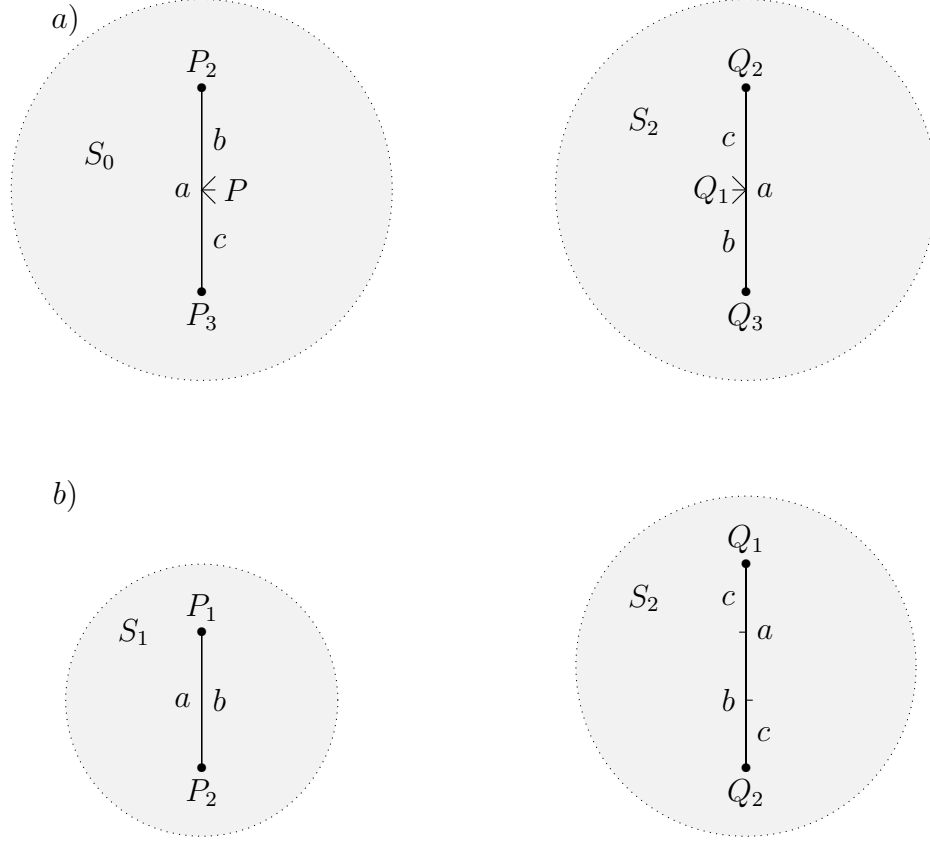
FIGURE 2. Surfaces in \mathcal{H}(-p, -q, p + q) .
