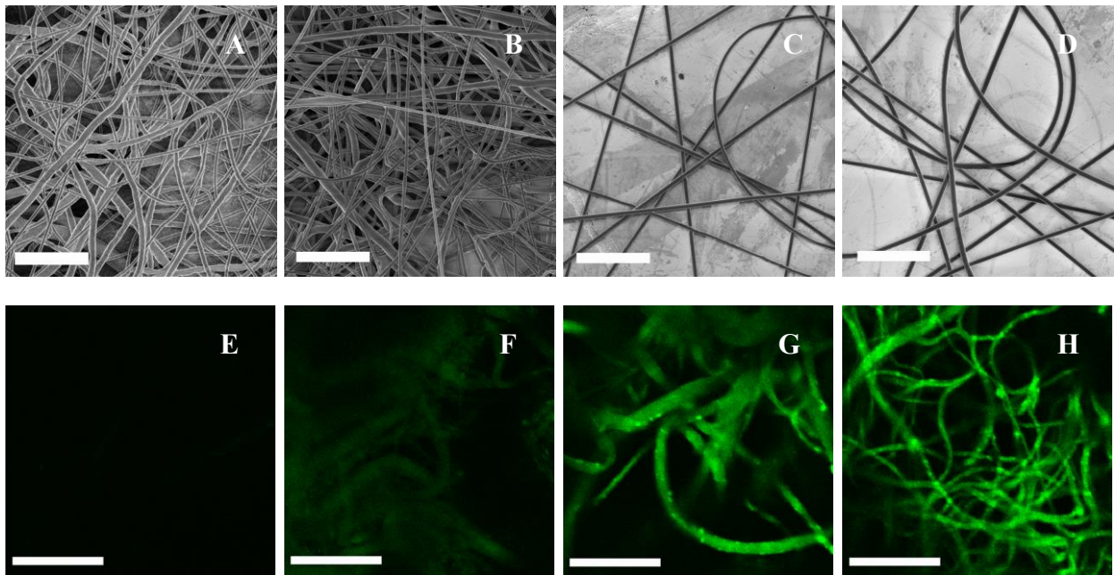
Figure 2. FESEM images (A-D) and fluorescent images (E-H) of f-PCL 80 fibers containing: 0 wt% (A,E), 20 wt % (B,F), 40 wt % (C,G) and 60 wt % (D,H) of PCL-N 3 . For fluorescence microscopy, prior observation, all samples were incubated with FITC-alkyne fluorophore and copper catalysts. Scale bar 10 \mu\text{m} (A-D) and 20 \mu\text{m} (E-H).
