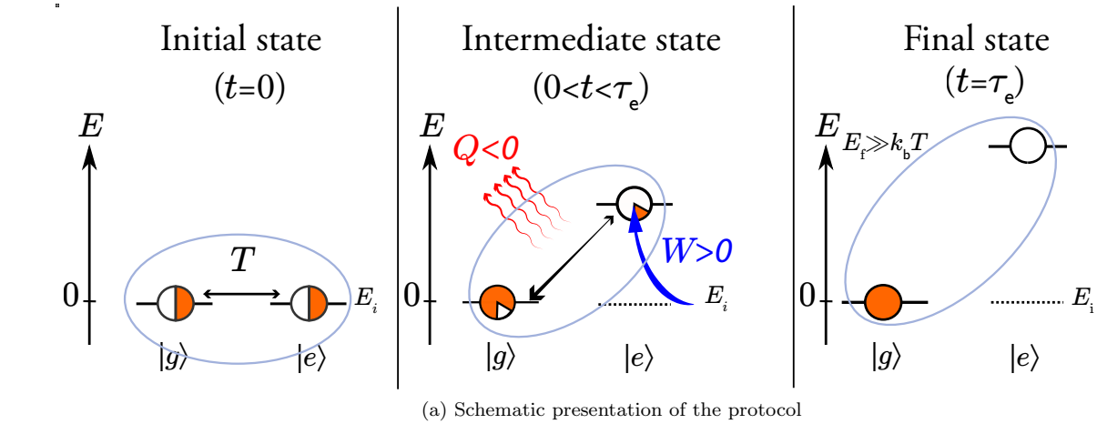
(a) Schematic presentation of the protocol
