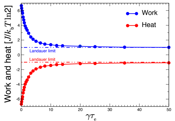
(c) Evolution of averaged work and heat
