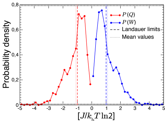
(b) Probability distribution of total heat Q(\tau_e) and work W(\tau_e)
