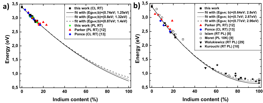
Fig. 6: Extrapolation of the In content dependence of the bandgap energy of InGaN alloys to the whole indium content range according to the different InN bandgap values, for a) strained and b) relaxed layers. Data obtained in this work and by other authors are shown for comparison.
